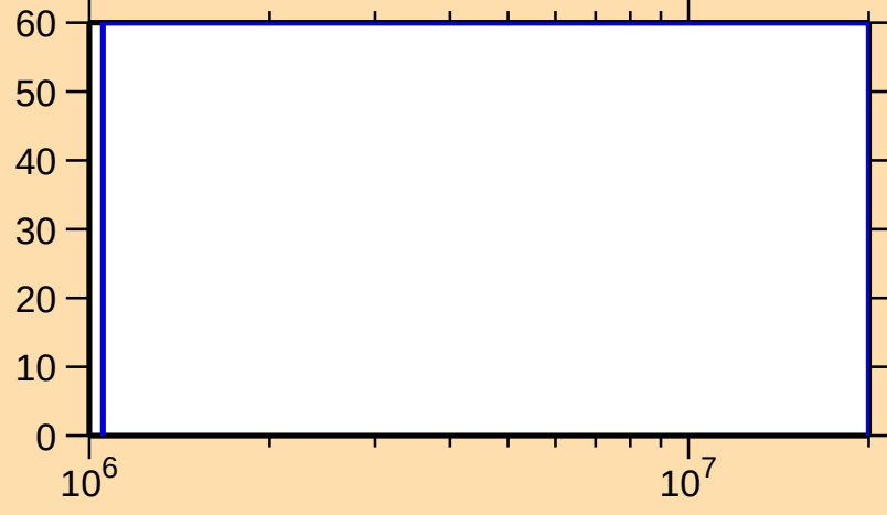
\Delta\sigma/\sigma vs. E for ^{71}\text{Br}(n,n\text{cont.})
