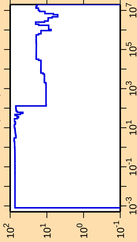
\Delta\sigma/\sigma vs. E for ^{71}\text{Br}(n,\text{el.})
