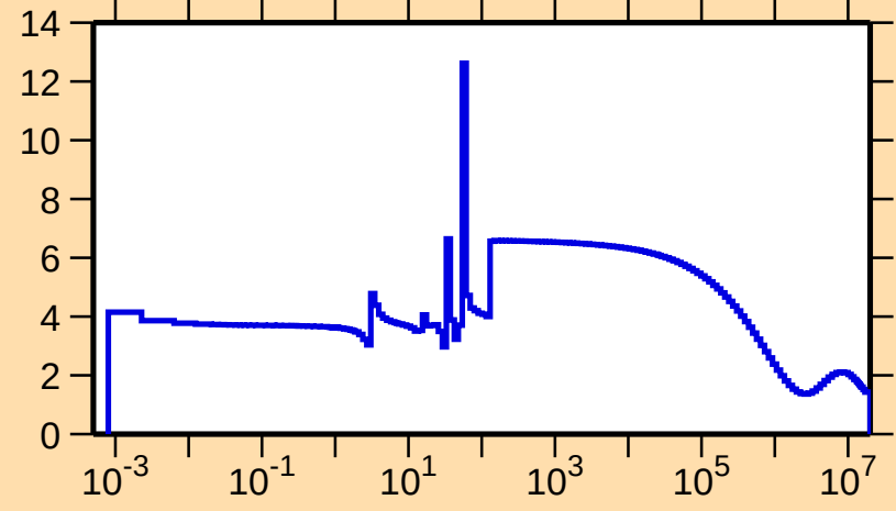
\sigma vs. E for ^{71}\text{Br}(n,\text{el.})
