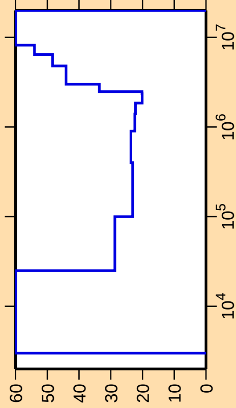
\Delta\sigma/\sigma vs. E for ^{71}\text{Br}(n,p)
