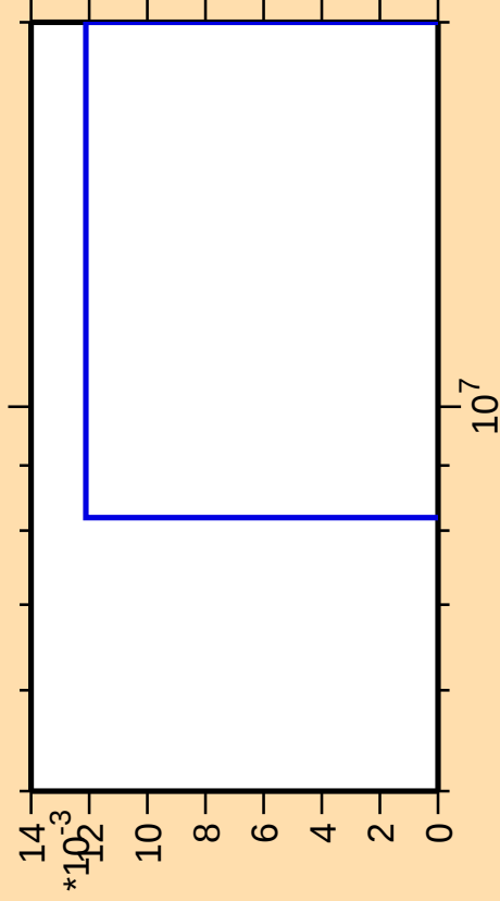
\Delta\sigma/\sigma vs. E for ^{71}\text{Br}(n,nt)
