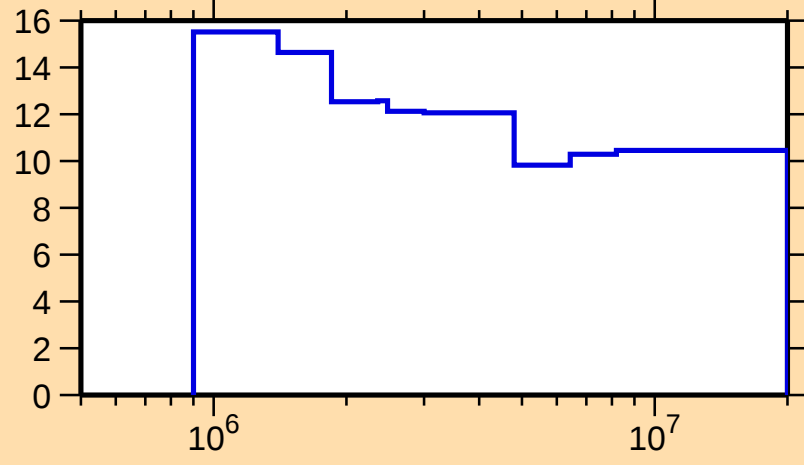
\Delta\sigma/\sigma vs. E for ^{71}\text{Br}(\text{n},\text{nonel.})
