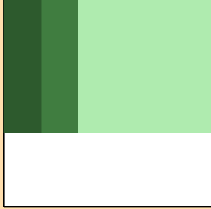
\Delta\sigma/\sigma vs. E for ^{71}\text{Br}(n,\text{tot.})
