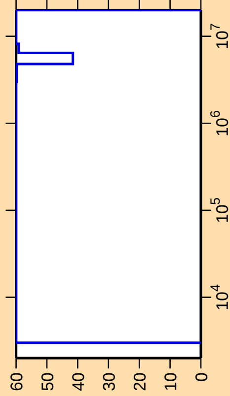
\Delta\sigma/\sigma vs. E for ^{71}\text{Br}(n,\gamma)
