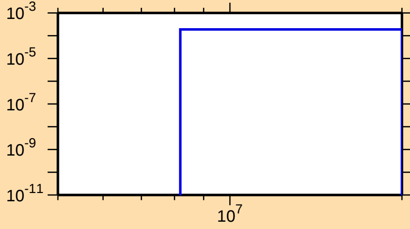
\sigma vs. E for ^{71}\text{Br}(n,t)
