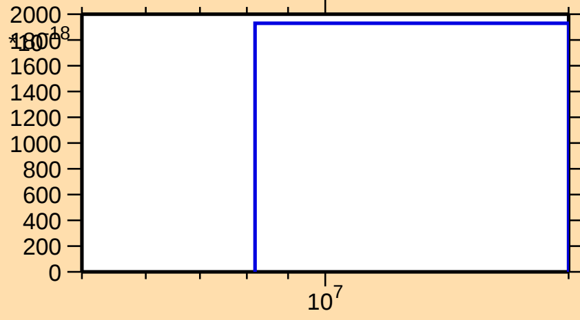
\sigma vs. E for ^{71}\text{Br}(n,nt)
