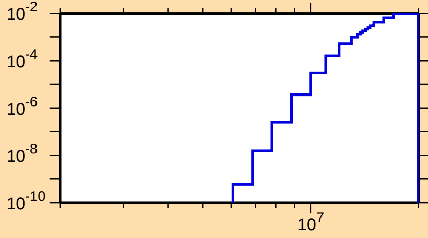
\sigma vs. E for ^{72}\text{Br}(n,\text{He}3)
