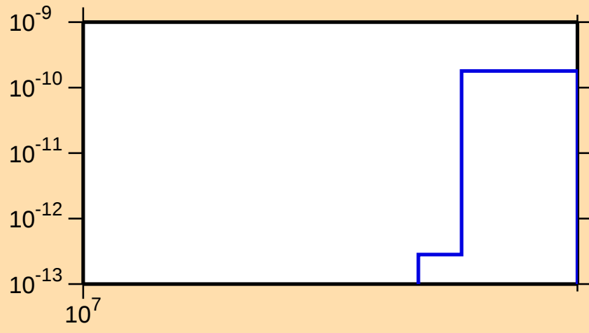
\sigma vs. E for ^{72}\text{Br}(n,2n\alpha)
