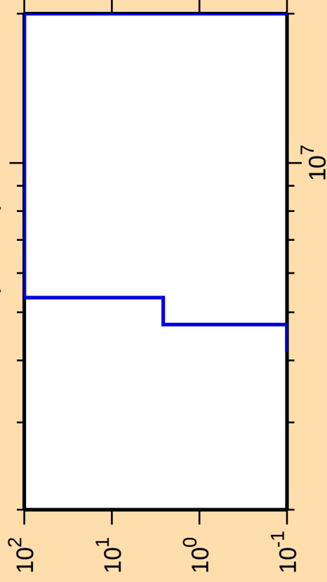
\Delta\sigma/\sigma vs. E for ^{72}\text{Br}(n,\text{He}3)
