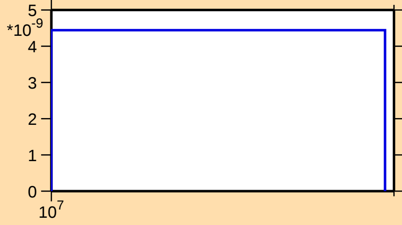
\sigma vs. E for ^{72}\text{Br}(\text{mt } 34)
