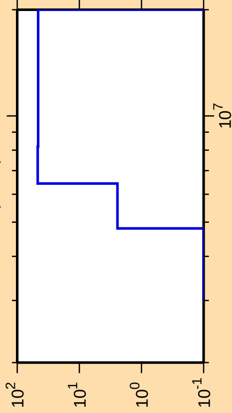
\Delta\sigma/\sigma vs. E for ^{72}\text{Br}(n,n\alpha)
