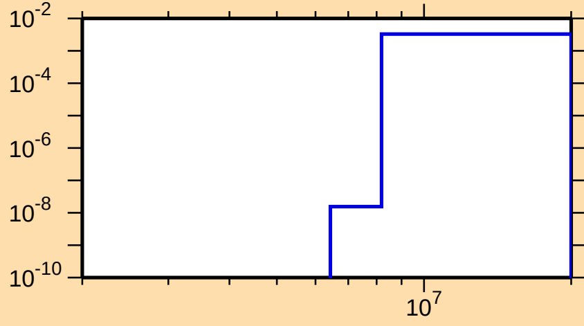
\sigma vs. E for ^{72}\text{Br}(n,n\alpha)
