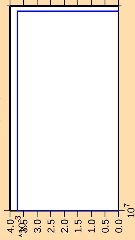
\Delta\sigma/\sigma vs. E for ^{72}\text{Br}(n,\text{nt})
