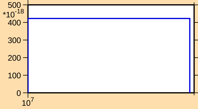
\sigma vs. E for ^{72}\text{Br}(n,\text{nt})
