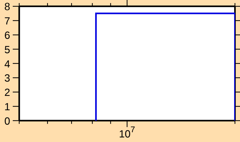
\Delta\sigma/\sigma vs. E for ^{72}\text{Br}(n,\text{nonel.})
