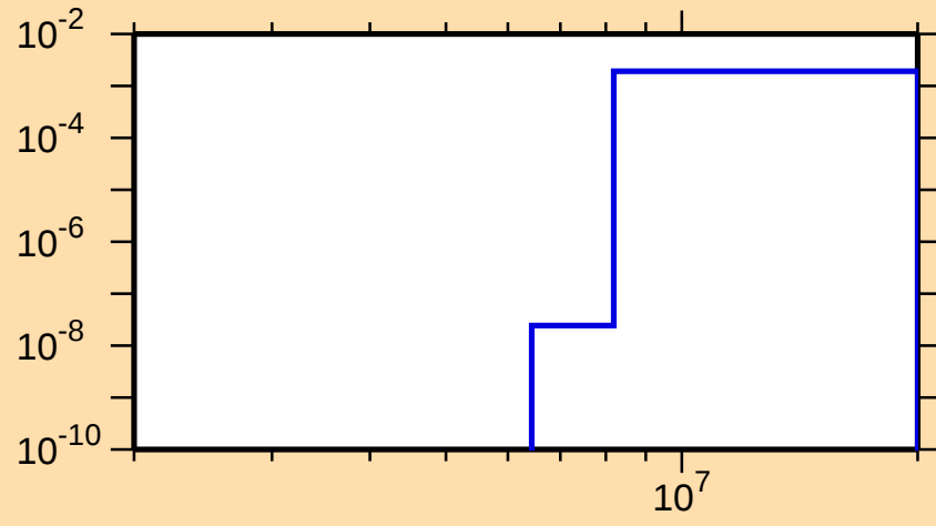
\sigma vs. E for ^{72}\text{Br}(n,\text{He}3)
