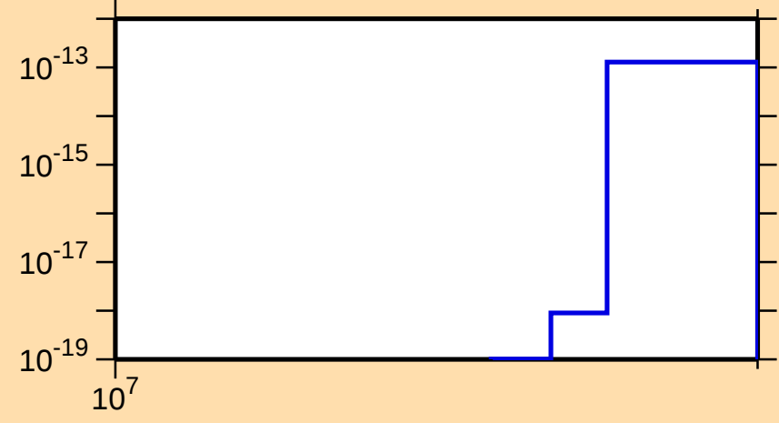
\sigma vs. E for ^{73}\text{Br}(n,2n\alpha)
