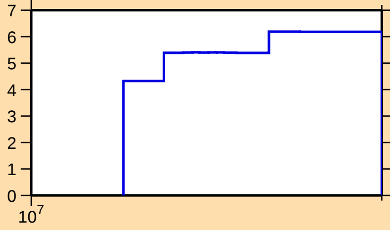
\Delta\sigma/\sigma vs. E for ^{73}\text{Br}(n,\text{tot.})
