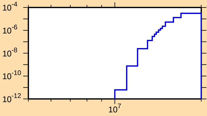
\sigma vs. E for ^{73}\text{Br}(\text{mt117})
