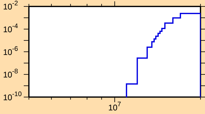
\sigma vs. E for ^{73}\text{Br}(n,\text{pd})
