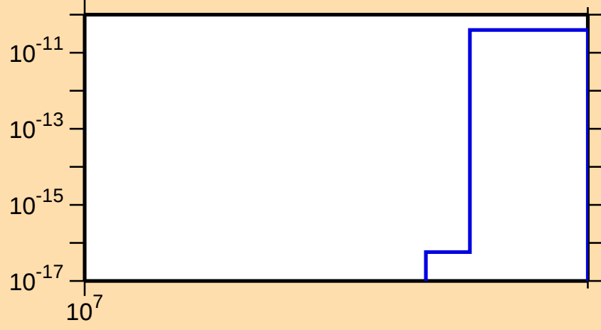
\sigma vs. E for ^{73}\text{Br}(\text{mt } 34)
