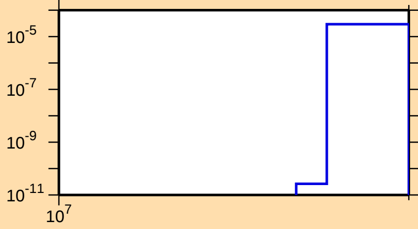
\sigma vs. E for ^{73}\text{Br}(n,2np)
