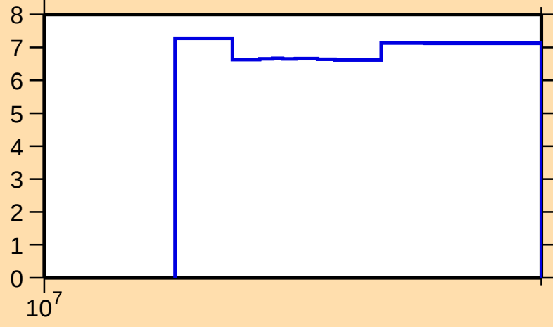
\Delta\sigma/\sigma vs. E for ^{73}\text{Br}(n,\text{nonel.})
