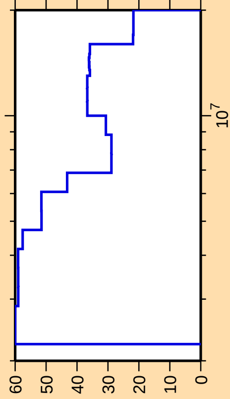
\Delta\sigma/\sigma vs. E for ^{73}\text{Br}(n,\gamma)
