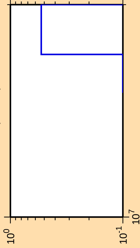
\Delta\sigma/\sigma vs. E for ^{73}\text{Br}(n,2n\alpha)
