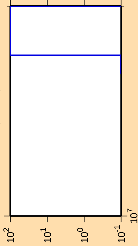
\Delta\sigma/\sigma vs. E for ^{73}\text{Br}(\text{mt } 34)
