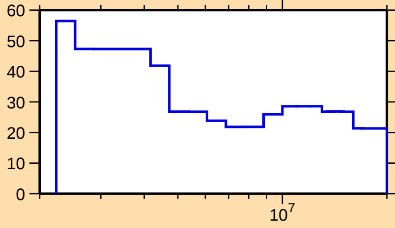
\Delta\sigma/\sigma vs. E for ^{73}\text{Br}(n,n\text{cont.})
