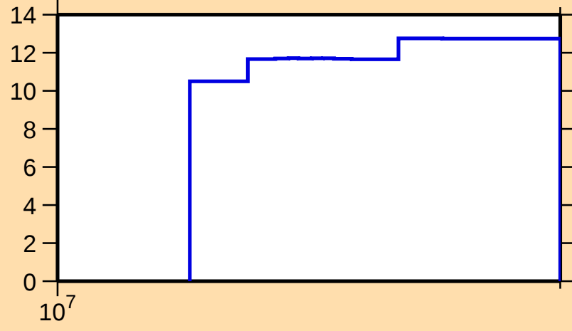
\Delta\sigma/\sigma vs. E for ^{73}\text{Br}(n,\text{inel.})
