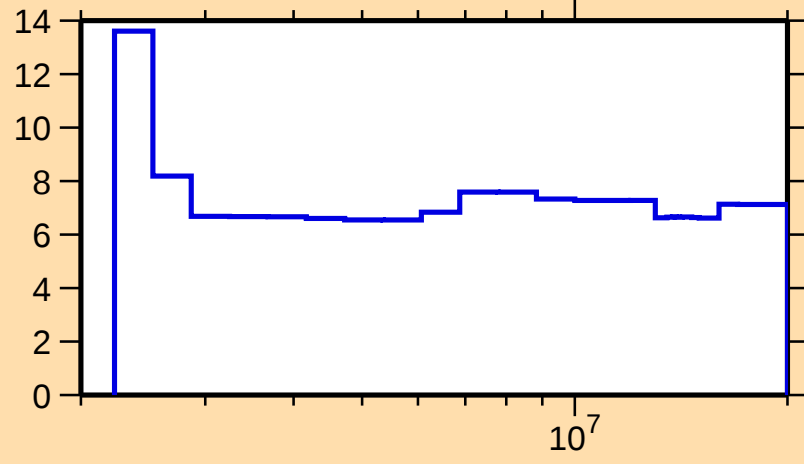
\Delta\sigma/\sigma vs. E for ^{73}\text{Br}(n,\text{nonel.})
