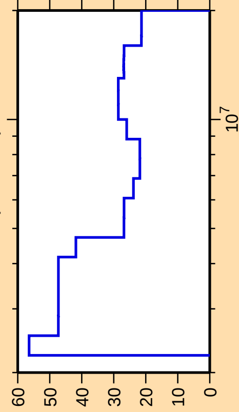
\Delta\sigma/\sigma vs. E for ^{73}\text{Br}(n,n\text{cont.})
