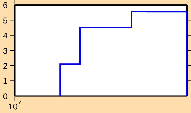
\Delta\sigma/\sigma vs. E for ^{73}\text{Br}(n,\text{el.})
