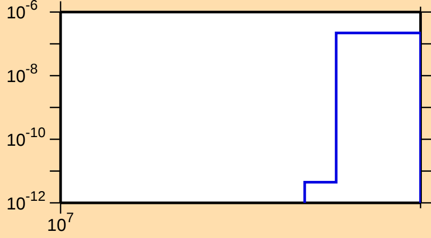
\sigma vs. E for ^{73}\text{Br}(n,\text{pt})
