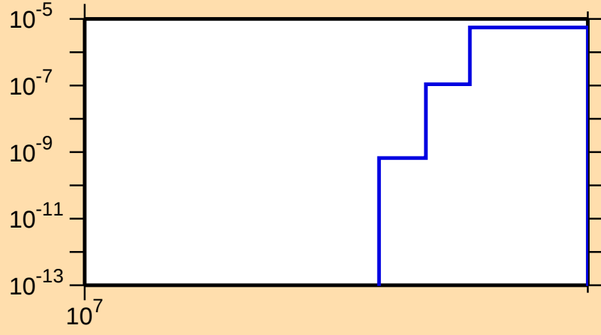
\sigma vs. E for ^{73}\text{Br}(n,\text{nd})
