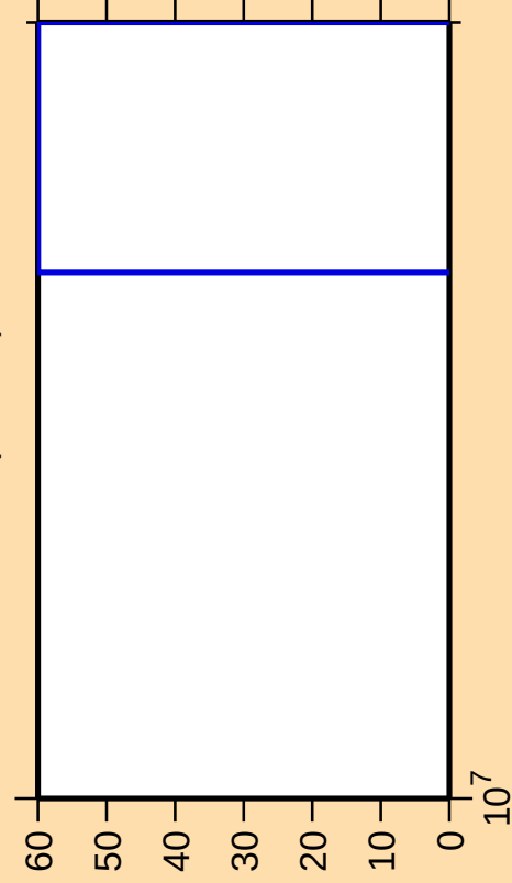
\Delta\sigma/\sigma vs. E for ^{74}\text{Br}(\text{mt } 34)
