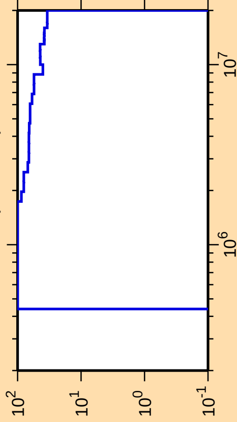
\Delta\sigma/\sigma vs. E for ^{74}\text{Br}(n,\text{ncont.})
