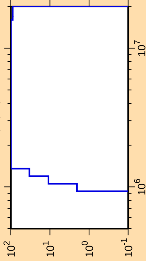
\Delta\sigma/\sigma vs. E for ^{74}\text{Br}(n,p\alpha)
