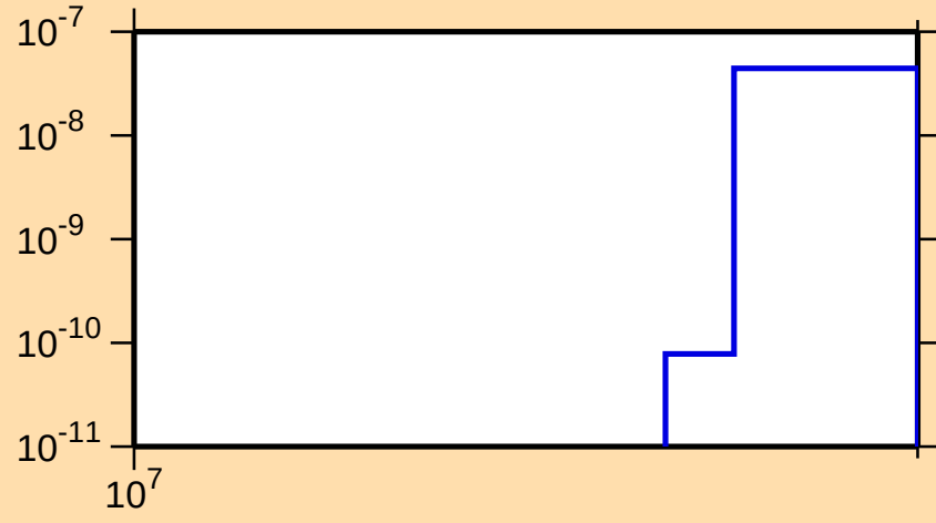
\sigma vs. E for ^{74}\text{Br}(\text{mt } 34)
