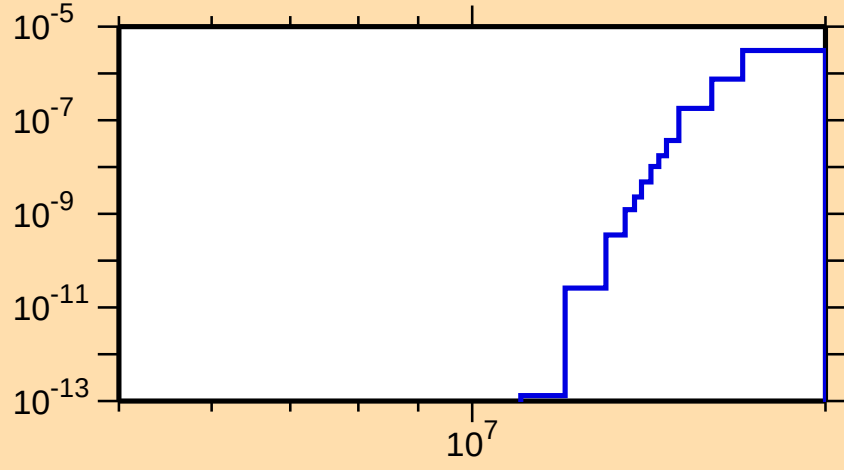
\sigma vs. E for ^{74}\text{Br}(\text{mt117})
