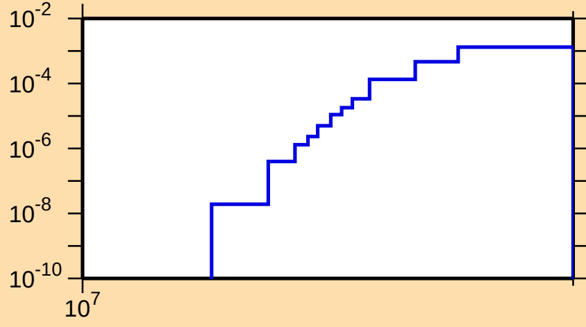
\sigma vs. E for ^{74}\text{Br}(n,\text{nd})
