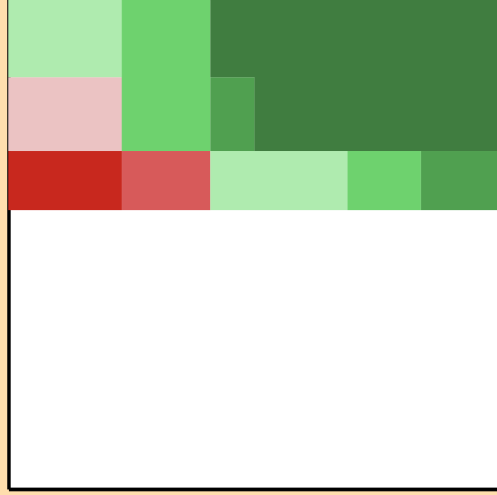
\Delta\sigma/\sigma vs. E for ^{74}\text{Br}(n,\text{el.})
