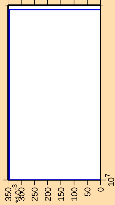
\Delta\sigma/\sigma vs. E for ^{74}\text{Br}(n,\text{nt})
