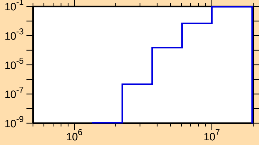
\sigma vs. E for ^{74}\text{Br}(n,p\alpha)
