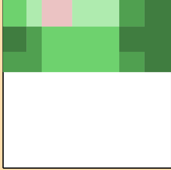
\Delta\sigma/\sigma vs. E for ^{74}\text{Br}(n,\text{tot.})
