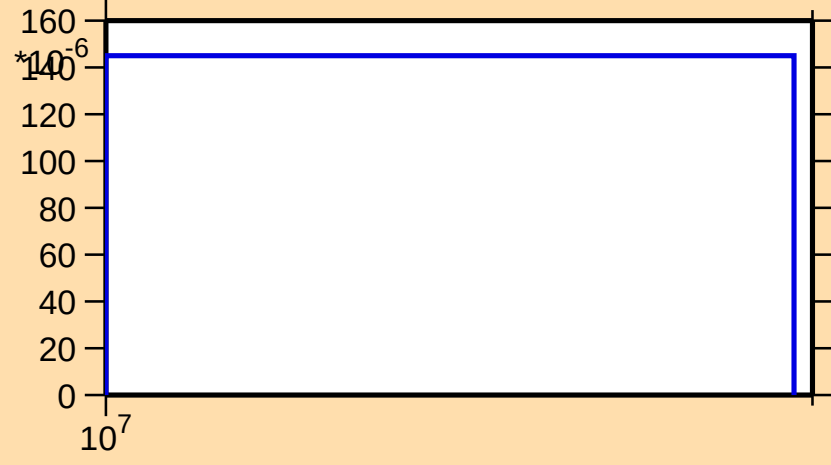
\sigma vs. E for ^{74}\text{Br}(n,2np)
