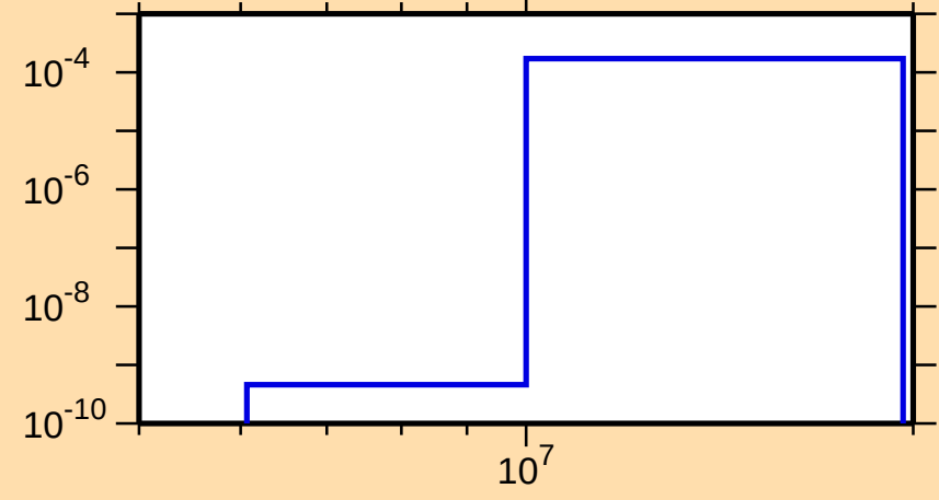
\sigma vs. E for ^{74}\text{Br}(n,\text{He}3)
