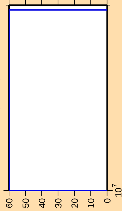
\Delta\sigma/\sigma vs. E for ^{74}\text{Br}(\text{mt } 45)
