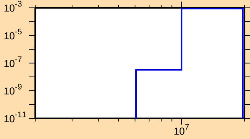
\sigma vs. E for ^{74}\text{Br}(n,t)
