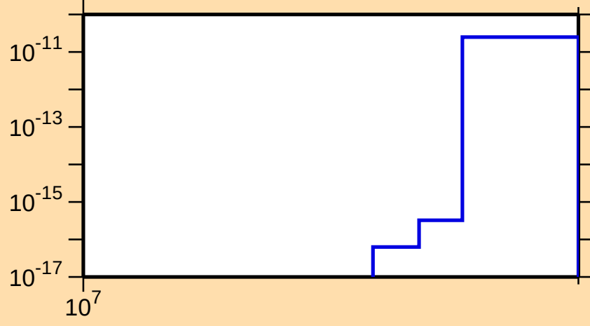
\sigma vs. E for ^{75}\text{Br}(n,\text{pt})
