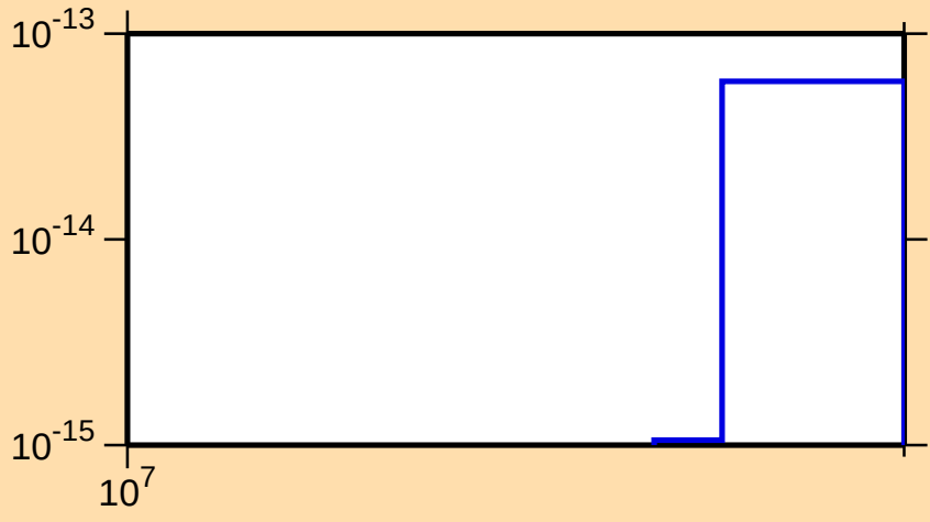
\sigma vs. E for ^{75}\text{Br}(\text{mt } 34)
