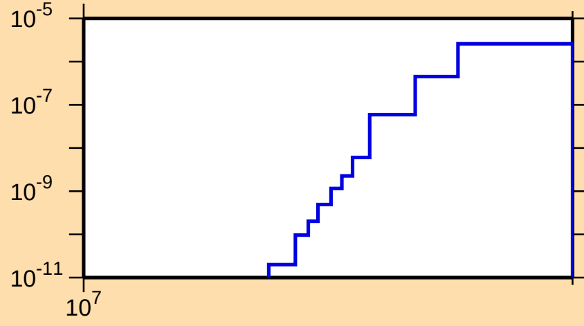
\sigma vs. E for ^{75}\text{Br}(\text{mt117})
