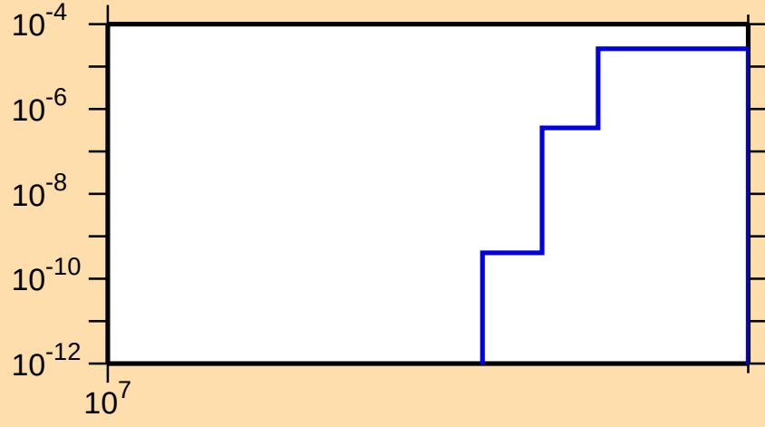
\sigma vs. E for ^{75}\text{Br}(n,\text{nd})
