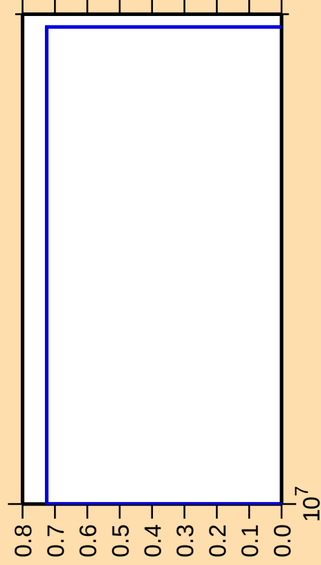
\Delta\sigma/\sigma vs. E for ^{75}\text{Br}(n,\text{pt})
