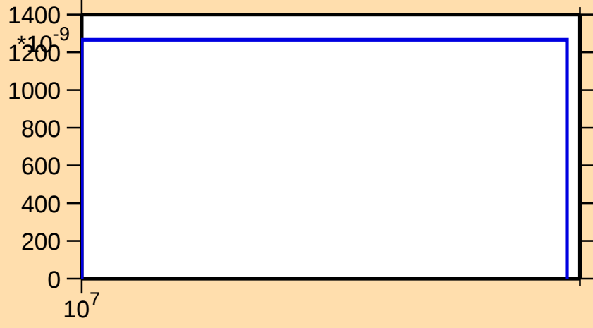
\sigma vs. E for ^{75}\text{Br}(n,\text{pd})
