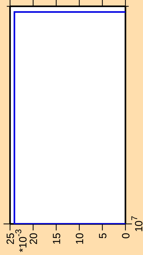
\Delta\sigma/\sigma vs. E for ^{75}\text{Br}(n,2n\alpha)
