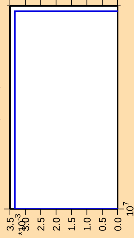
\Delta\sigma/\sigma vs. E for ^{75}\text{Br}(\text{mt } 34)
