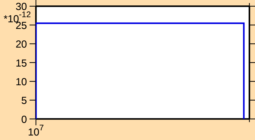
\sigma vs. E for ^{75}\text{Br}(n,nt)
