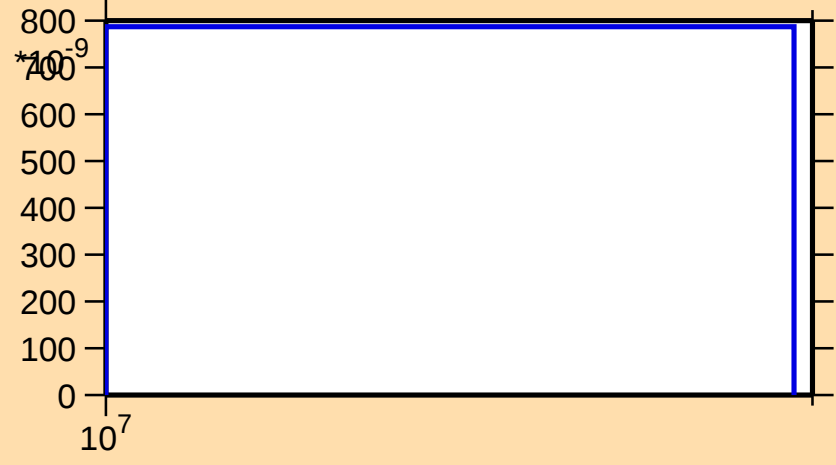
\sigma vs. E for ^{75}\text{Br}(n,2np)
