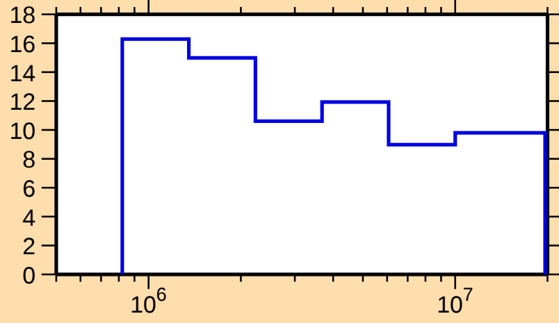
\Delta\sigma/\sigma vs. E for ^{75}\text{Br}(n,\text{el.})
