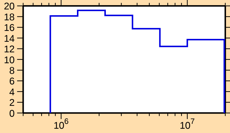
\Delta\sigma/\sigma vs. E for ^{75}\text{Br}(n,\text{nonel.})
