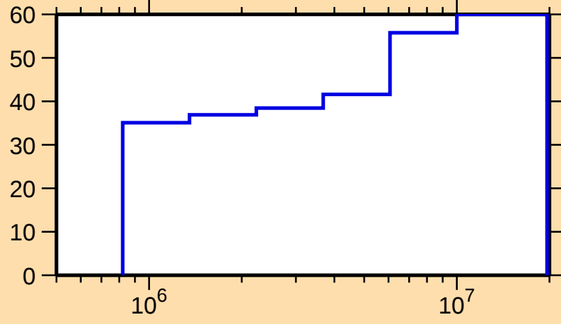
\Delta\sigma/\sigma vs. E for ^{75}\text{Br}(n,\text{inel.})
