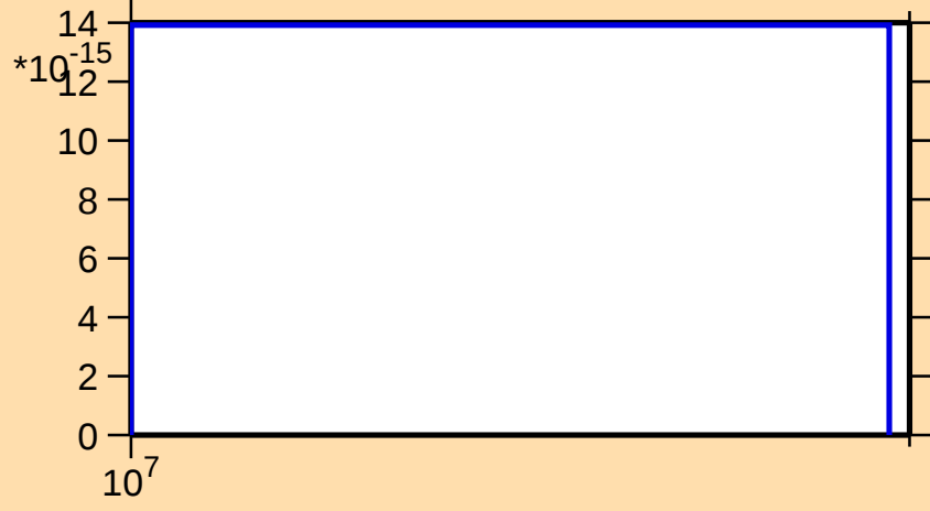
\sigma vs. E for ^{75}\text{Br}(n,2n\alpha)
