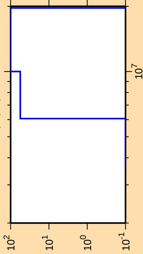
\Delta\sigma/\sigma vs. E for ^{75}\text{Br}(n,p\alpha)
