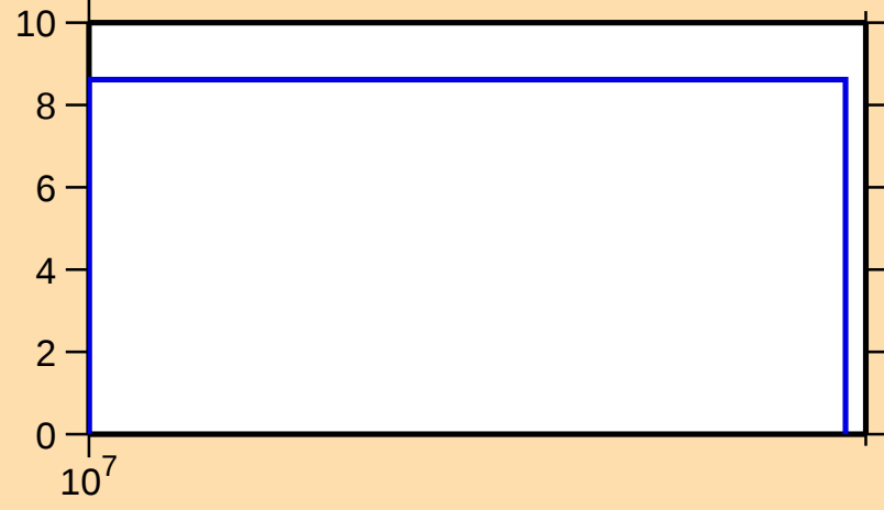
\Delta\sigma/\sigma vs. E for ^{75}\text{Br}(n,\text{tot.})
