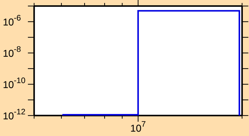
\sigma vs. E for ^{75}\text{Br}(n,\text{He3})
