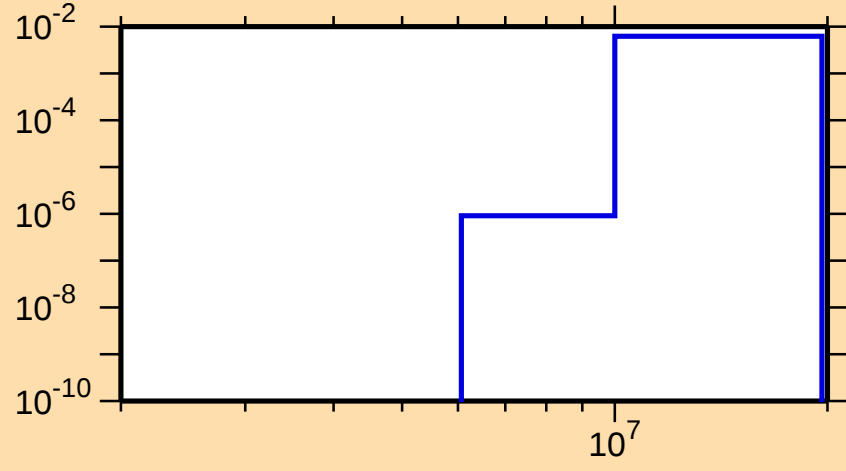
\sigma vs. E for ^{75}\text{Br}(n,p\alpha)
