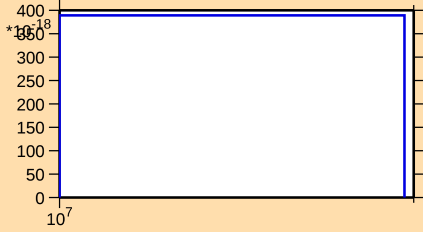
\sigma vs. E for ^{75}\text{Br}(\text{mt } 34)
