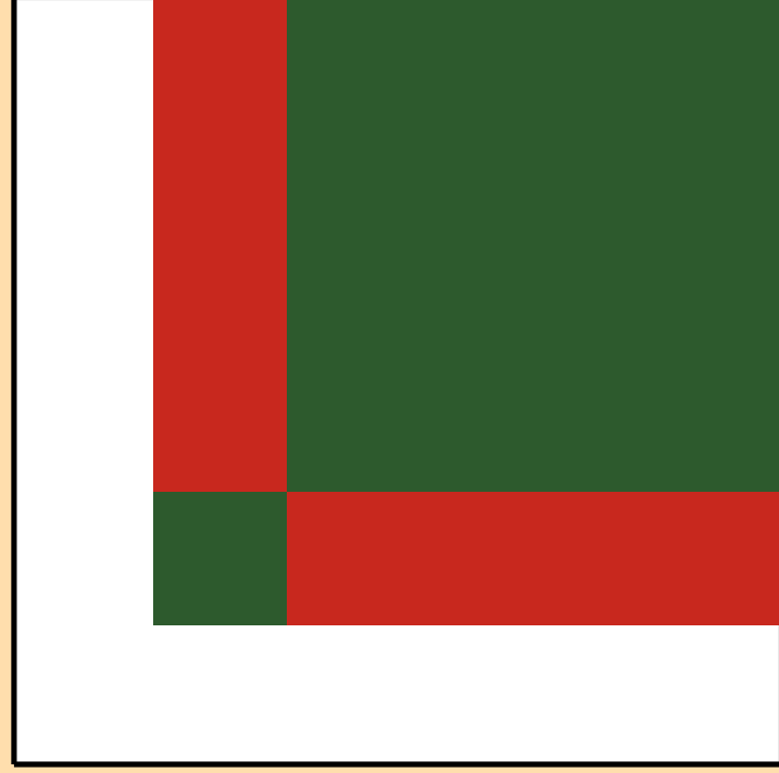
\sigma vs. E for ^{75}\text{Br}(n,n\alpha)
