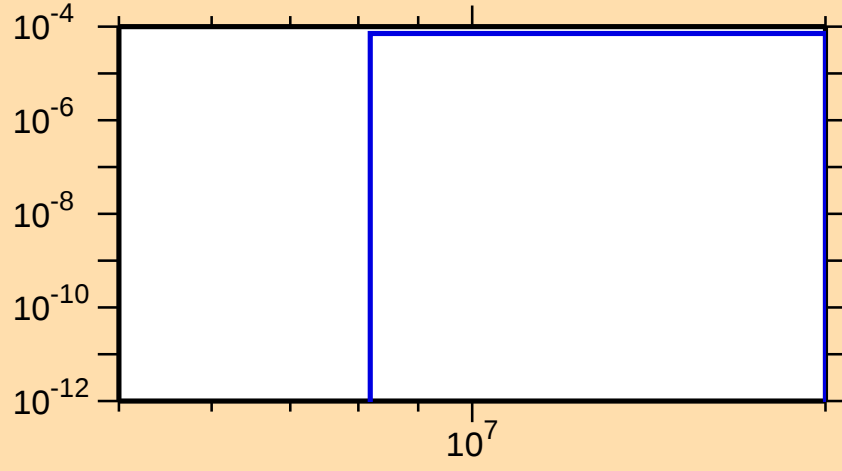
\sigma vs. E for ^{75}\text{Br}(n,t)
