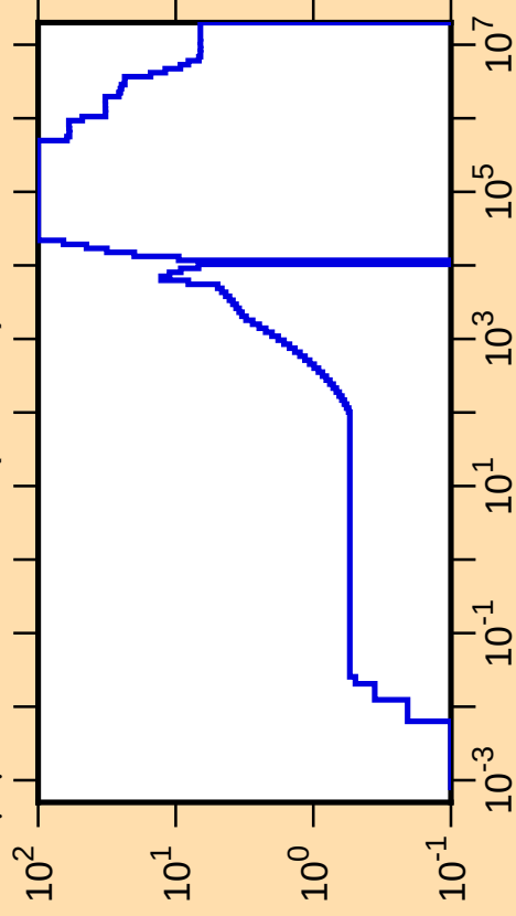
\Delta\mu/\mu vs. E for ^{77}\text{Br}(\text{mt251})
