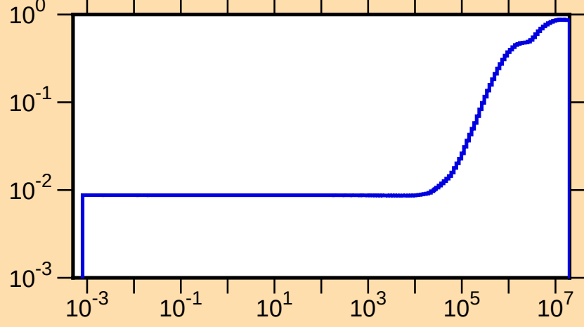
\mu vs. E for ^{77}\text{Br}(\text{mt251})
