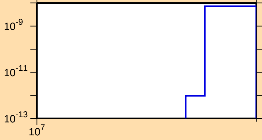
\sigma vs. E for ^{77}\text{Br}(n,nt)
