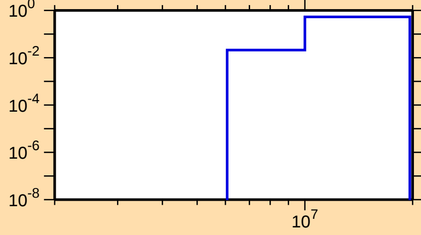
\sigma vs. E for ^{77}\text{Br}(n,np)
