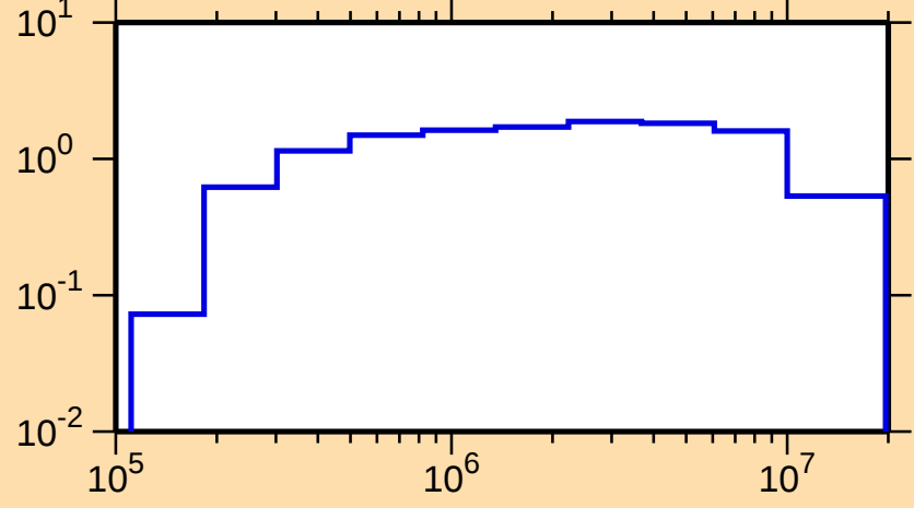
\sigma vs. E for ^{77}\text{Br}(n,\text{inel.})
