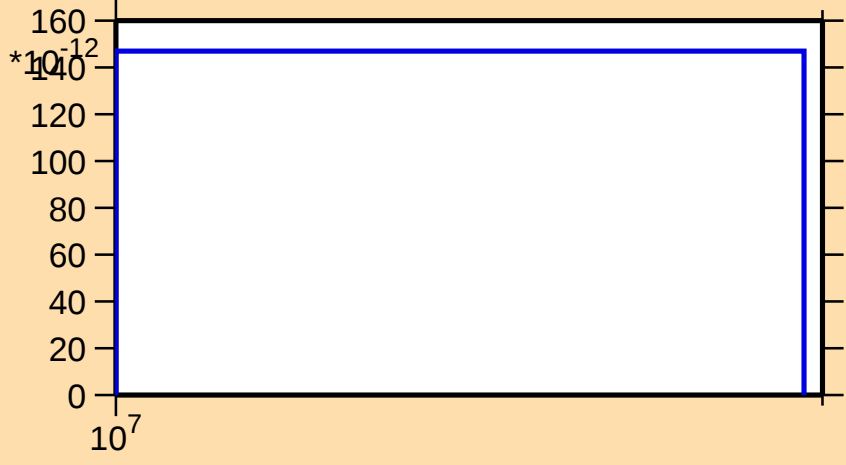
\sigma vs. E for ^{77}\text{Br}(\text{mt } 45)
