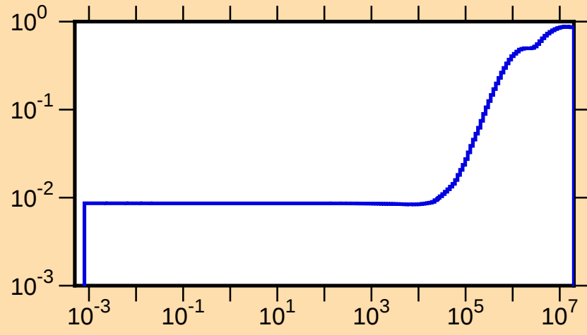
\mu vs. E for ^{78}\text{Br}(\text{mt251})
