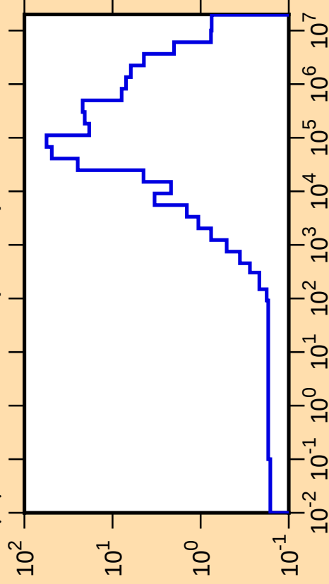
\Delta\mu/\mu vs. E for ^{78}\text{Br}(\text{mt251})
