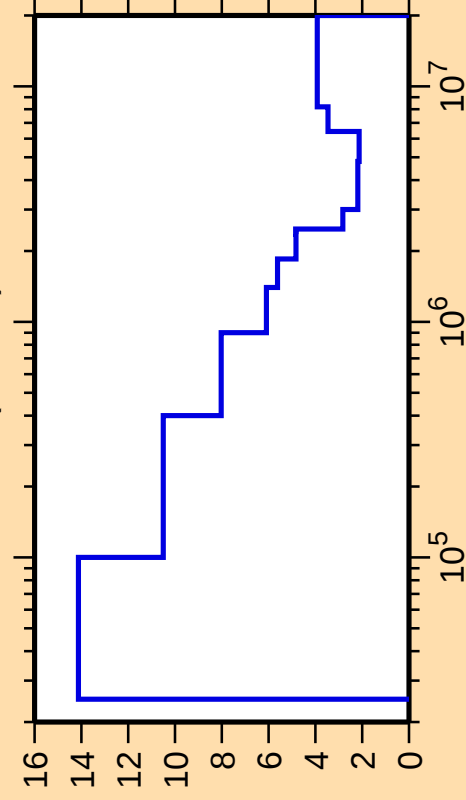
\Delta\sigma/\sigma vs. E for ^{78}\text{Br}(\text{n,inel.})
