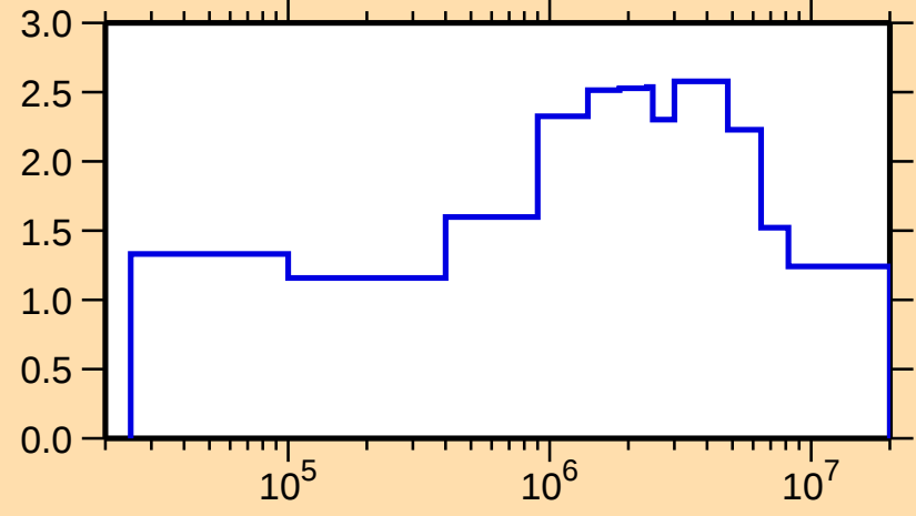
\Delta\sigma/\sigma vs. E for ^{78}\text{Br}(\text{n,el.})
