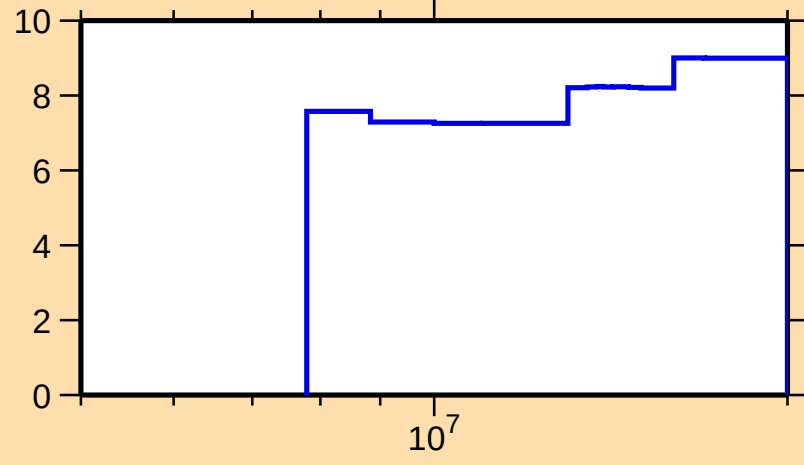
\Delta\sigma/\sigma vs. E for ^{80}\text{Br}(n,\text{nonel.})
