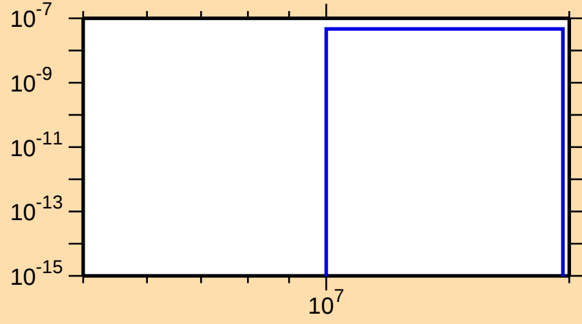
\sigma vs. E for ^{80}\text{Br}(n,p\alpha)
