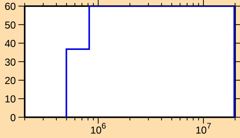
\Delta\sigma/\sigma vs. E for ^{80}\text{Br}(n,n_1)
