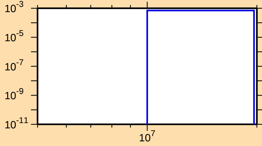
\sigma vs. E for ^{80}\text{Br}(n,n\alpha)
