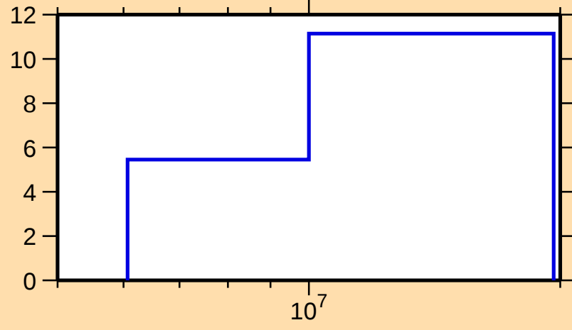
\Delta\sigma/\sigma vs. E for ^{80}\text{Br}(n,\text{tot.})
