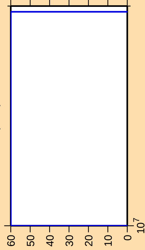
\Delta\sigma/\sigma vs. E for ^{81}\text{Br}(n,\text{nt})
