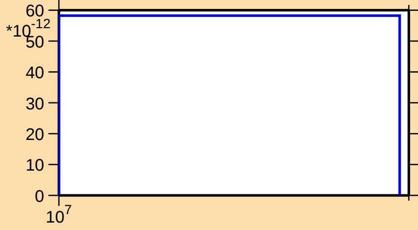
\sigma vs. E for ^{81}\text{Br}(n,\text{nt})
