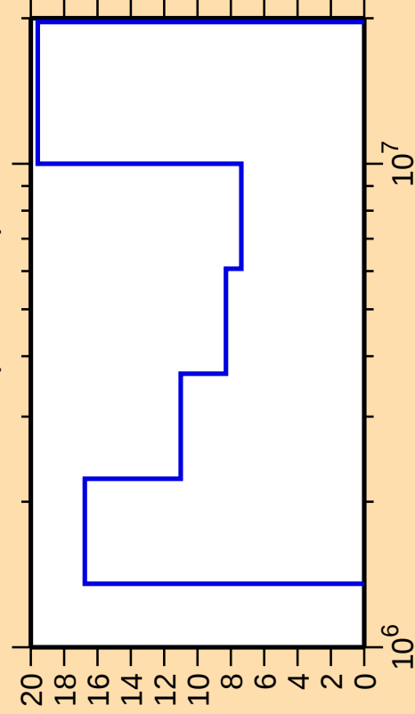
\Delta\sigma/\sigma vs. E for ^{81}\text{Br}(n,\text{ncont.})
