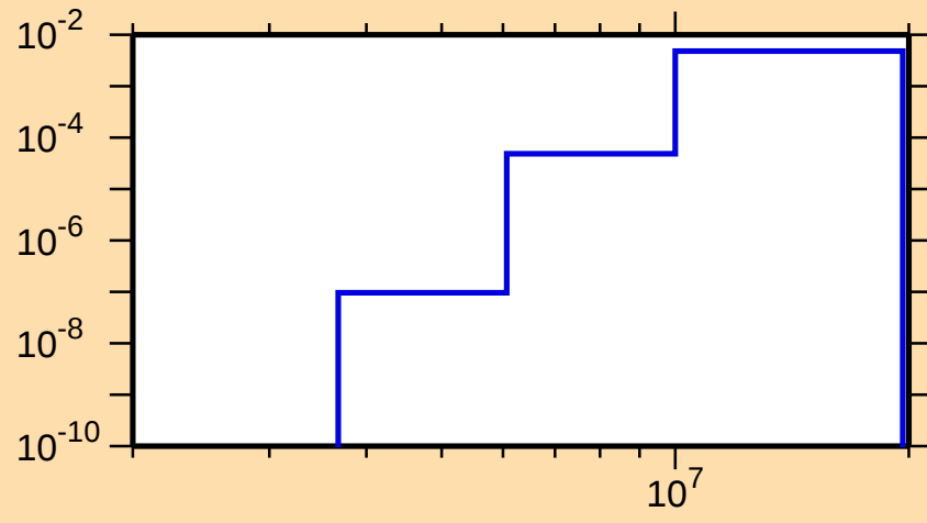
\sigma vs. E for ^{81}\text{Br}(n,\alpha)
