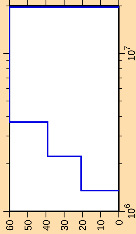
\Delta\sigma/\sigma vs. E for ^{81}\text{Br}(n,\gamma)
