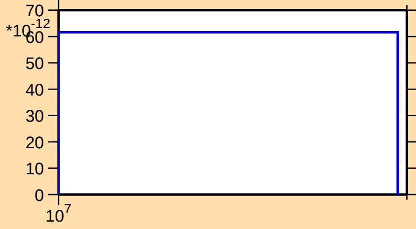
\sigma vs. E for ^{81}\text{Br}(n,2np)
