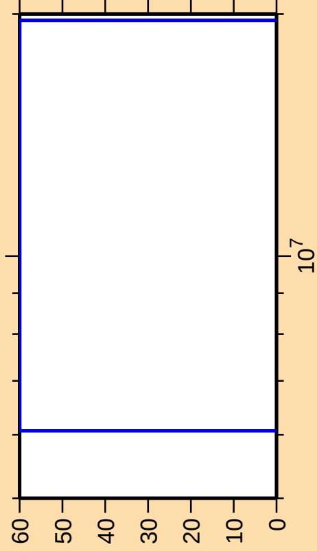
\Delta\sigma/\sigma vs. E for ^{81}\text{Br}(n,np)
