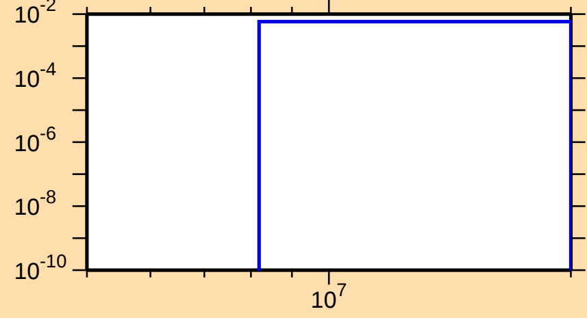
\sigma vs. E for ^{81}\text{Br}(n,np)
