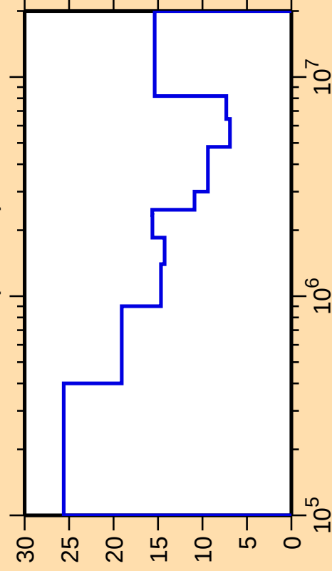
\Delta\sigma/\sigma vs. E for ^{81}\text{Br}(\text{n,inel.})
