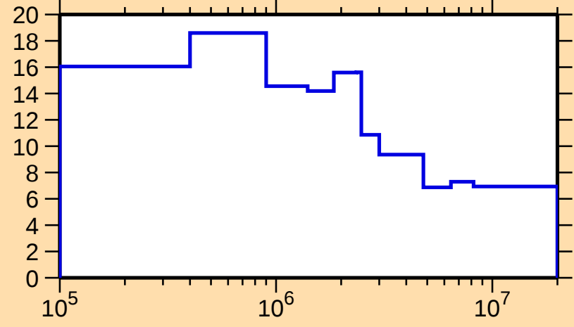
\Delta\sigma/\sigma vs. E for ^{81}\text{Br}(\text{n,nonel.})
