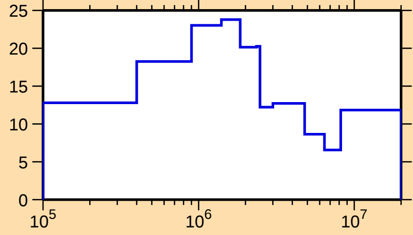
\Delta\sigma/\sigma vs. E for ^{81}\text{Br}(\text{n,el.})
