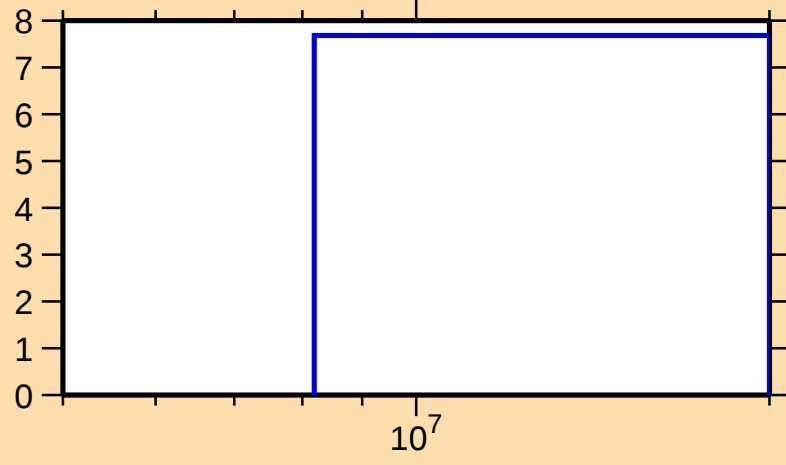
\Delta\sigma/\sigma vs. E for ^{81}\text{Br}(n,\text{tot.})
