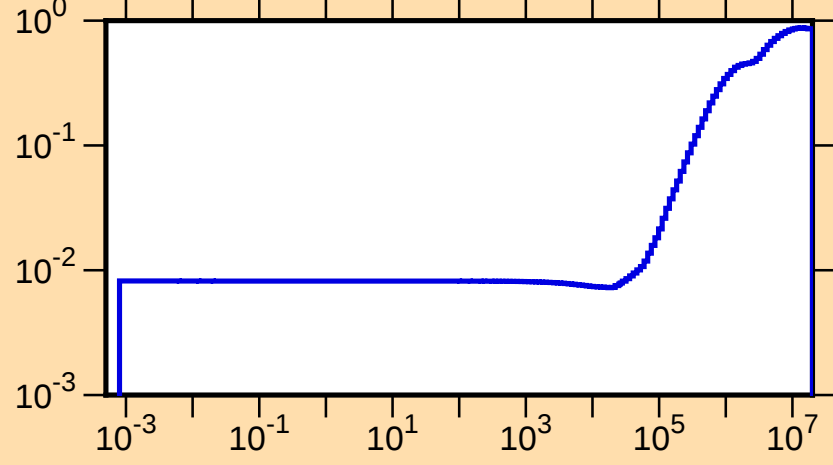
\mu vs. E for ^{82}\text{Br}(\text{mt251})
