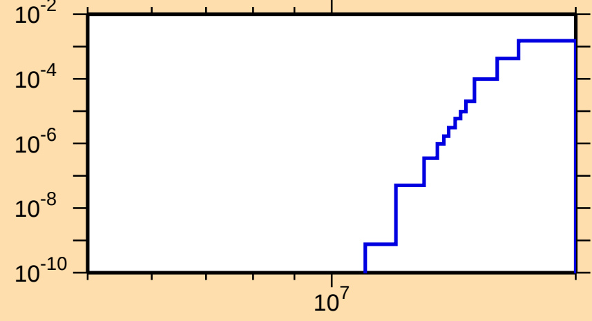
\sigma vs. E for ^{82}\text{Br}(n,n\alpha)
