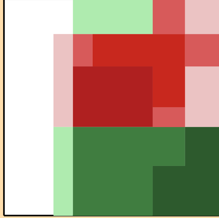
\Delta\sigma/\sigma vs. E for ^{82}\text{Br}(n,2n)
