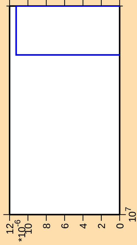
\Delta\sigma/\sigma vs. E for ^{82}\text{Br}(\text{mt } 34)
