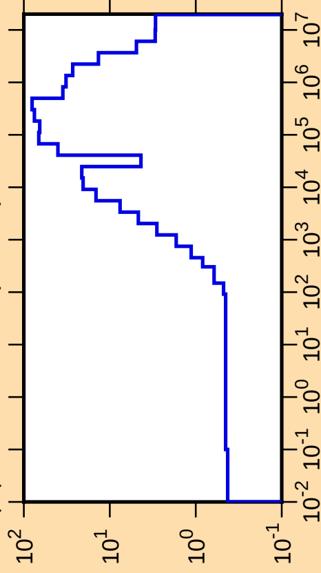
\Delta\mu/\mu vs. E for ^{82}\text{Br}(\text{mt251})
