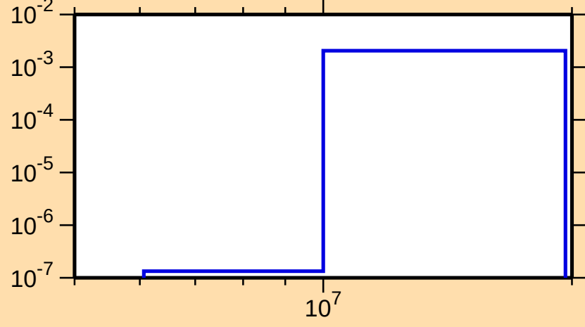
\sigma vs. E for ^{82}\text{Br}(n,d)
