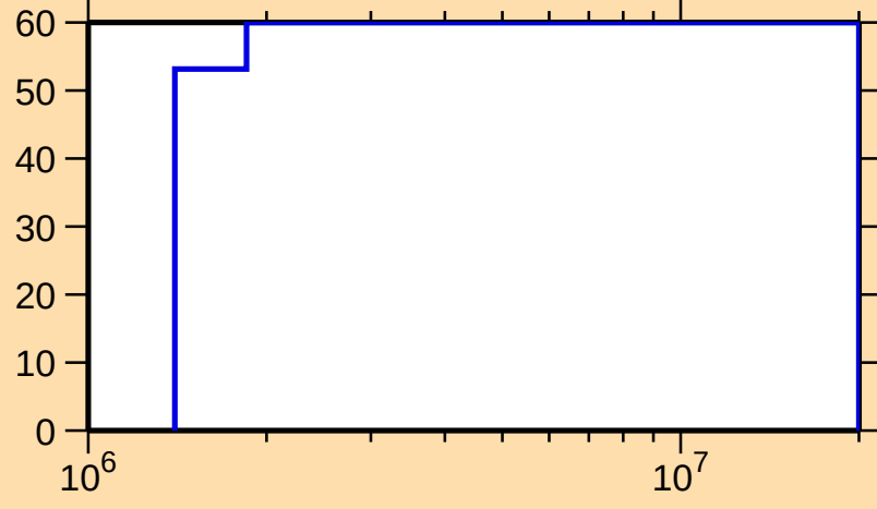
\Delta\sigma/\sigma vs. E for ^{82}\text{Br}(n,n_1)
