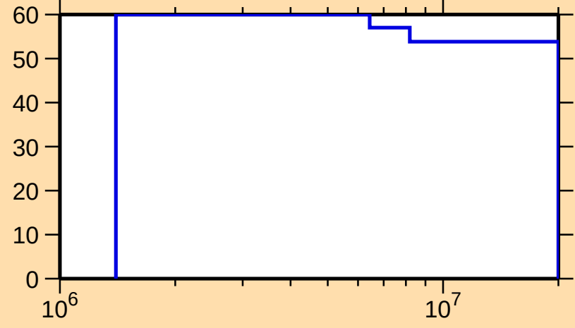
\Delta\sigma/\sigma vs. E for ^{82}\text{Br}(n,p)
