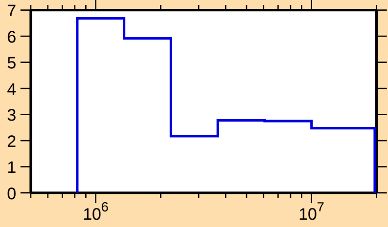
\Delta\sigma/\sigma vs. E for ^{82}\text{Br}(\text{n},\text{nonel.})
