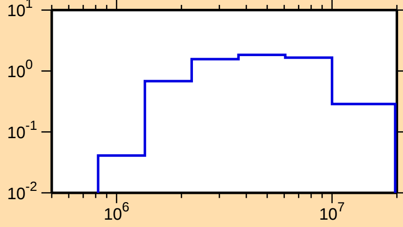
\sigma vs. E for ^{82}\text{Br}(n,n\text{cont.})
