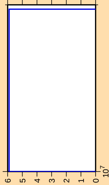
\Delta\sigma/\sigma vs. E for ^{82}\text{Br}(n,2n\alpha)
