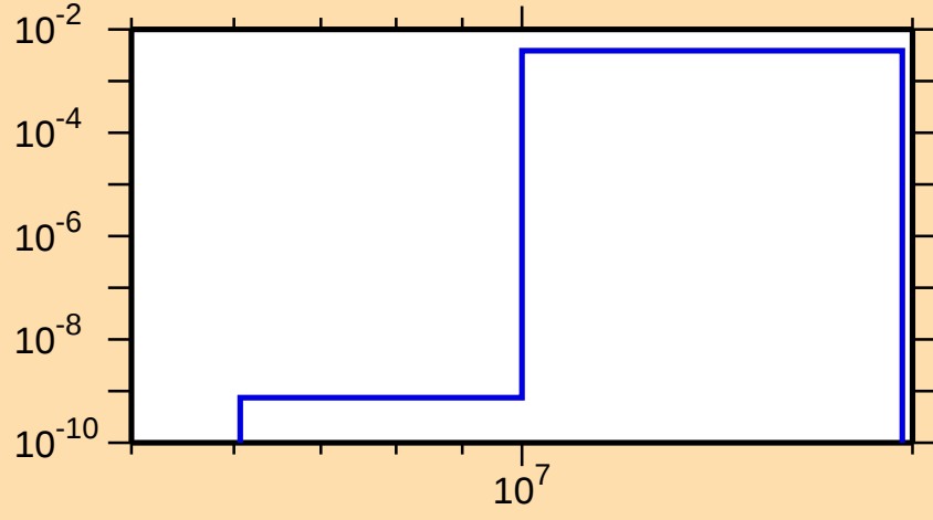
\sigma vs. E for ^{82}\text{Br}(n,np)
