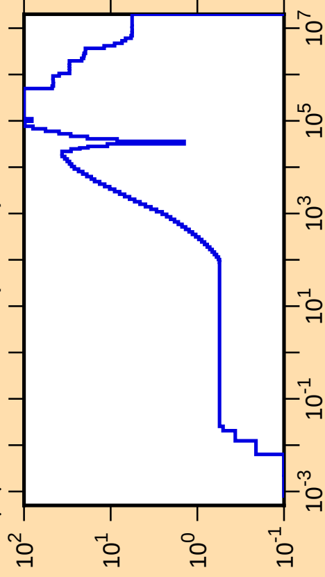
\Delta\mu/\mu vs. E for ^{83}\text{Br}(\text{mt251})
