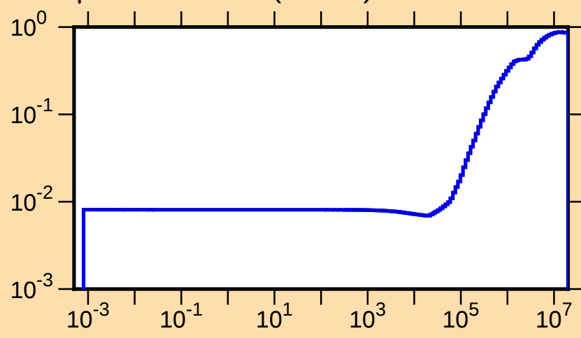
\mu vs. E for ^{83}\text{Br}(\text{mt251})
