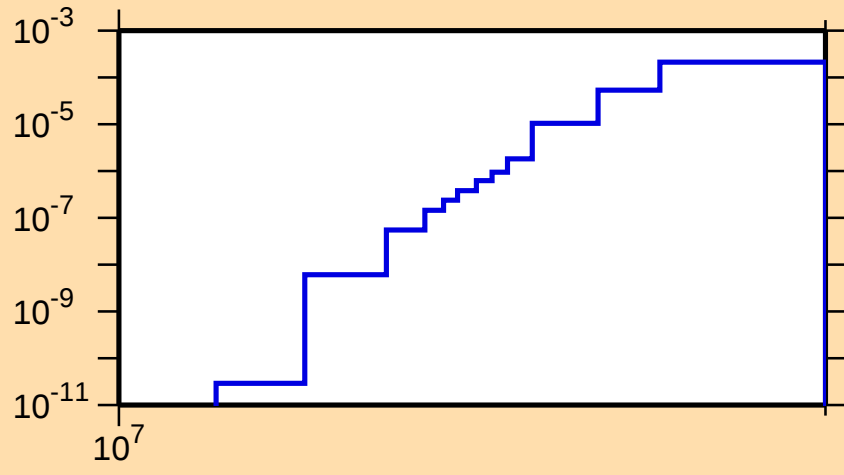
\sigma vs. E for ^{83}\text{Br}(n,t)
