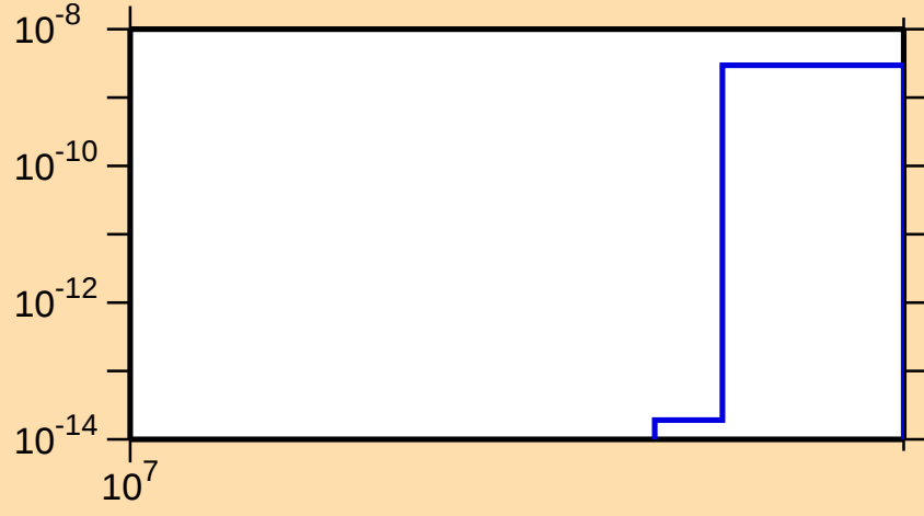
\sigma vs. E for ^{83}\text{Br}(n,\text{nt})
