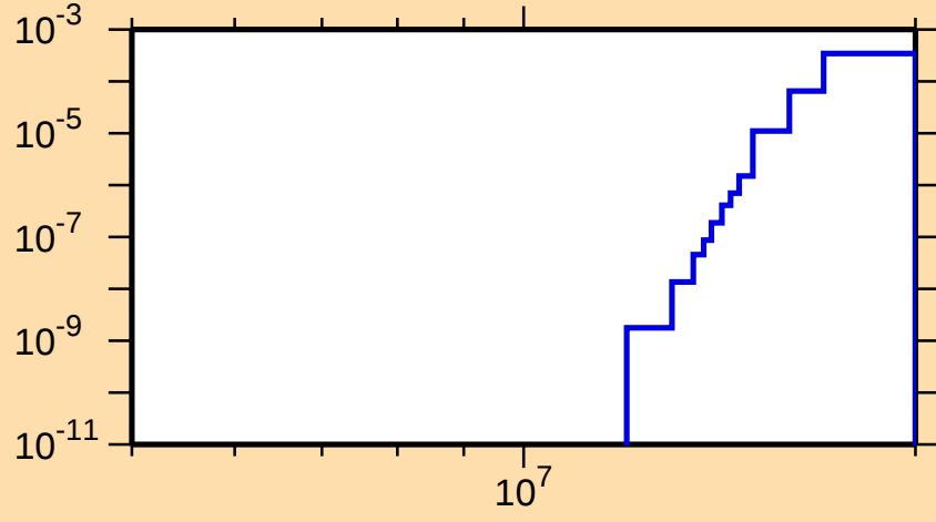
\sigma vs. E for ^{83}\text{Br}(n,\alpha)
