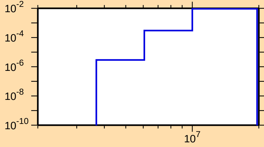
\sigma vs. E for ^{83}\text{Br}(n,p)
