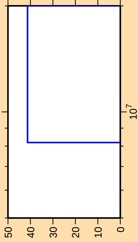
\Delta\sigma/\sigma vs. E for ^{83}\text{Br}(n,nt)
