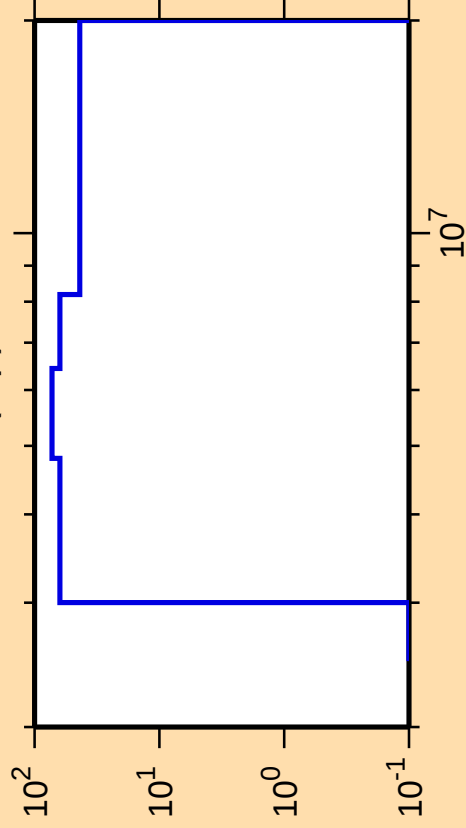
\Delta\sigma/\sigma vs. E for ^{83}\text{Br}(n,p)
