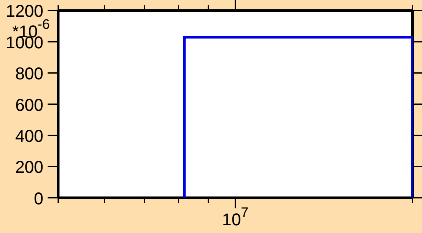
\sigma vs. E for ^{83}\text{Br}(n,np)
