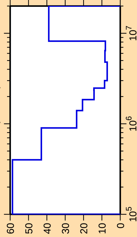
\Delta\sigma/\sigma vs. E for ^{83}\text{Br}(\text{n,inel.})
