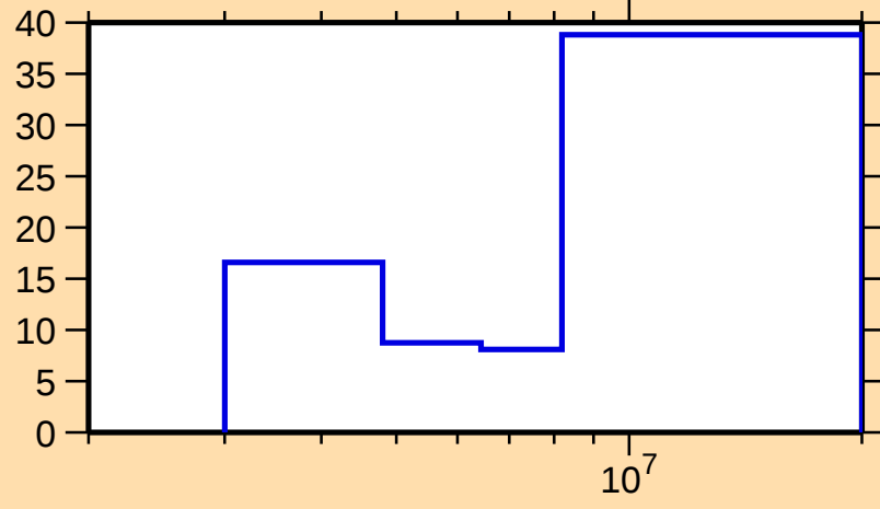
\Delta\sigma/\sigma vs. E for ^{83}\text{Br}(n,n\text{cont.})
