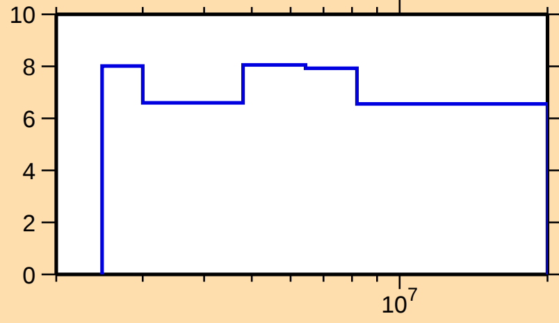
\Delta\sigma/\sigma vs. E for ^{83}\text{Br}(n,\text{nonel.})
