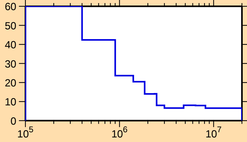
\Delta\sigma/\sigma vs. E for ^{83}\text{Br}(\text{n,nonel.})
