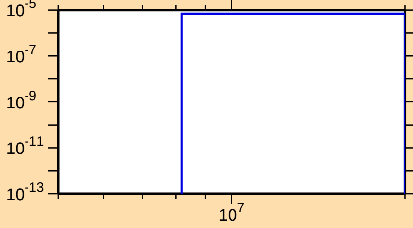
\sigma vs. E for ^{83}\text{Br}(n,n\alpha)
