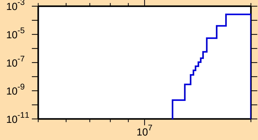
\sigma vs. E for ^{84}\text{Br}(n,\alpha)
