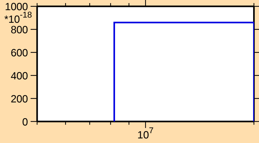
\sigma vs. E for ^{84}\text{Br}(n,p\alpha)
