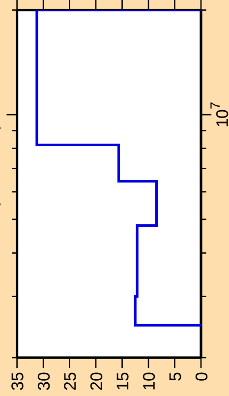
\Delta\sigma/\sigma vs. E for ^{84}\text{Br}(n,\text{ncont.})
