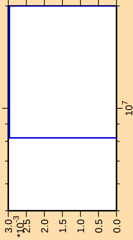
\Delta\sigma/\sigma vs. E for ^{84}\text{Br}(n,p\alpha)
