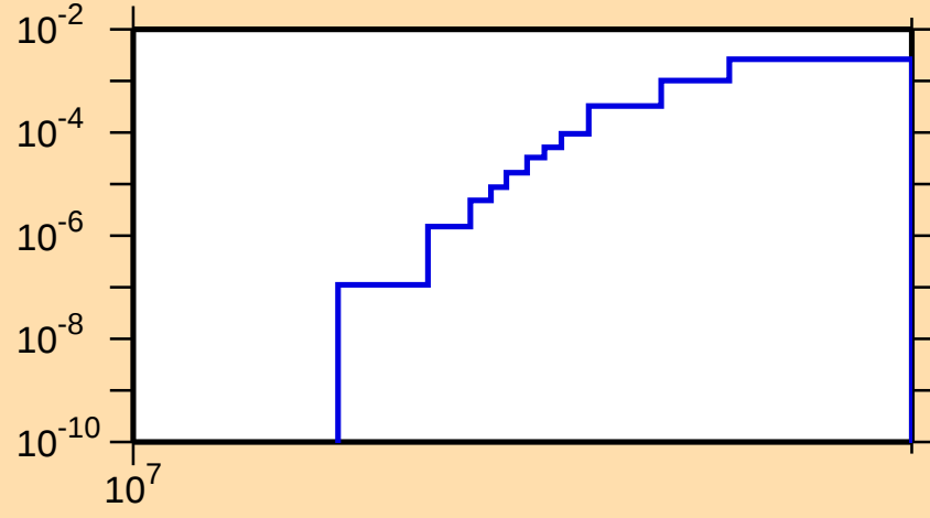
\sigma vs. E for ^{86}\text{Br}(n,np)
