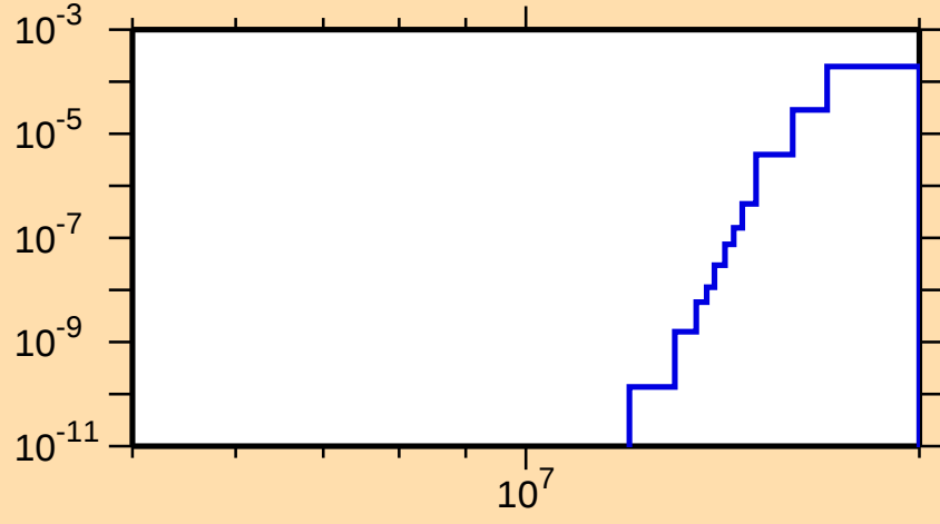
\sigma vs. E for ^{86}\text{Br}(n,\alpha)
