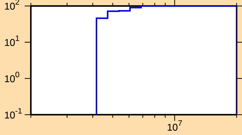
\Delta\sigma/\sigma vs. E for ^{86}\text{Br}(n,n_1)
