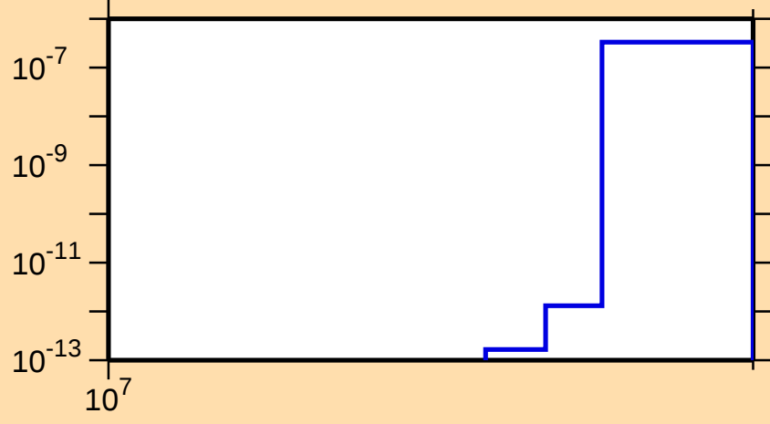
\sigma vs. E for ^{86}\text{Br}(n,nt)
