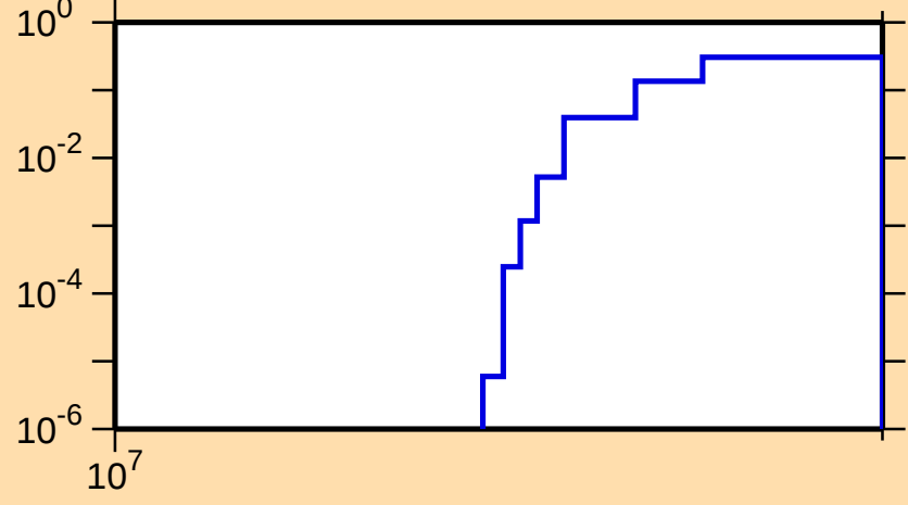
\sigma vs. E for ^{86}\text{Br}(n,3n)
