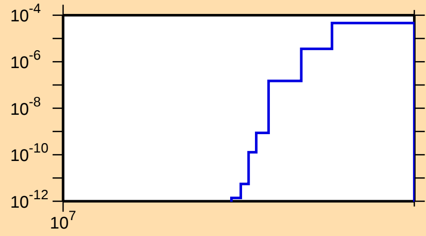
\sigma vs. E for ^{86}\text{Br}(n,\text{nd})
