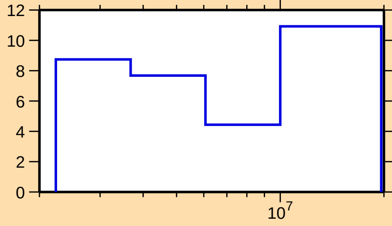
\Delta\sigma/\sigma vs. E for ^{86}\text{Br}(n,\text{tot.})
