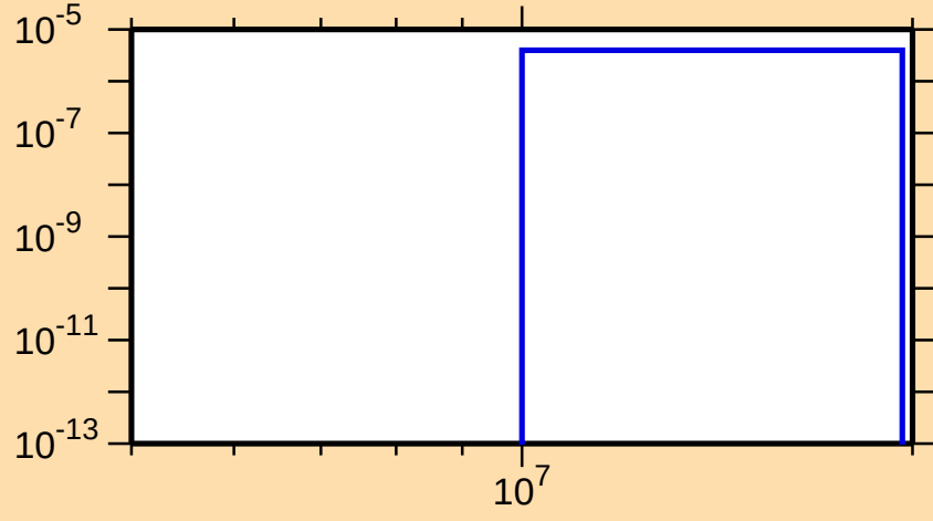
\sigma vs. E for ^{86}\text{Br}(n,n\alpha)
