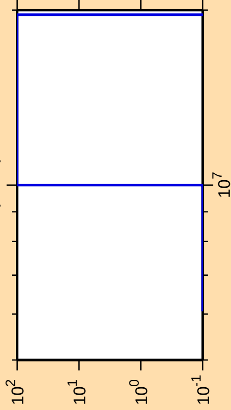
\Delta\sigma/\sigma vs. E for ^{86}\text{Br}(n,n\alpha)
