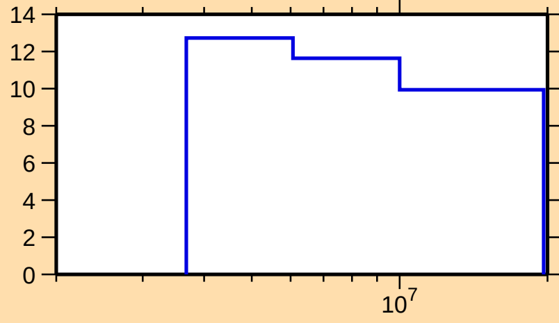
\Delta\sigma/\sigma vs. E for ^{86}\text{Br}(n,\text{nonel.})
