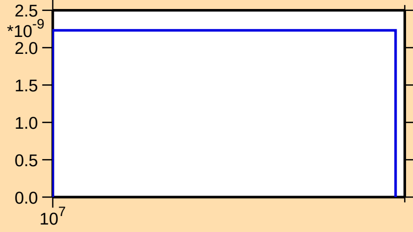
\sigma vs. E for ^{86}\text{Br}(n,\text{nt})
