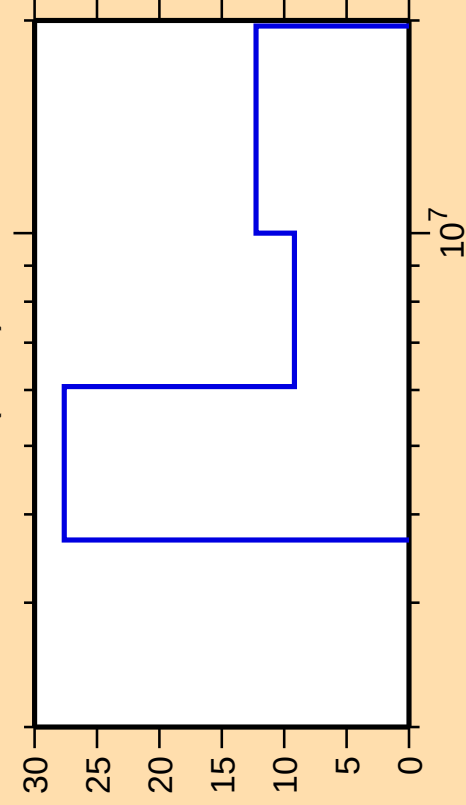
\Delta\sigma/\sigma vs. E for ^{86}\text{Br}(n,2n)
