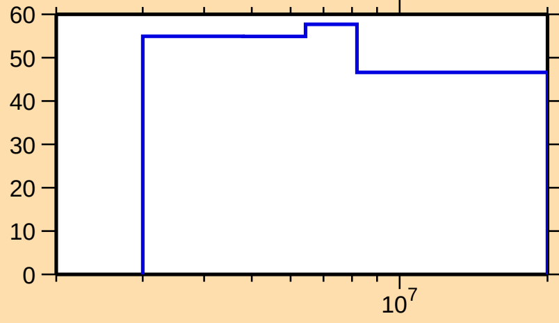
\Delta\sigma/\sigma vs. E for ^{86}\text{Br}(n,n\text{cont.})
