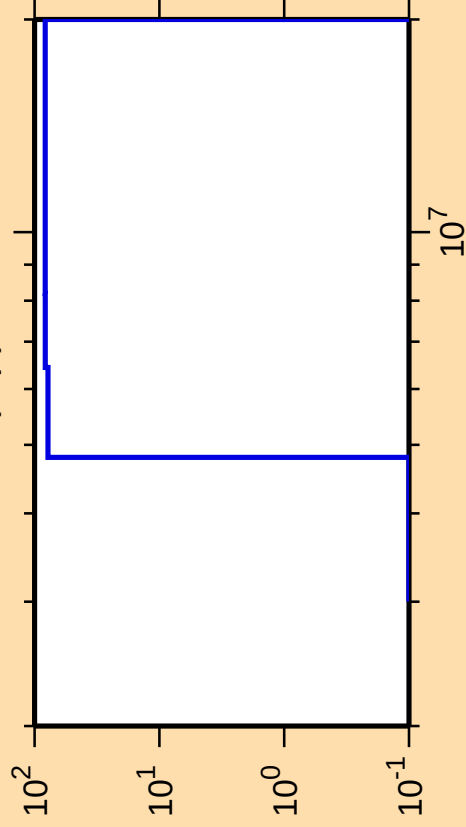
\Delta\sigma/\sigma vs. E for ^{86}\text{Br}(n,p)
