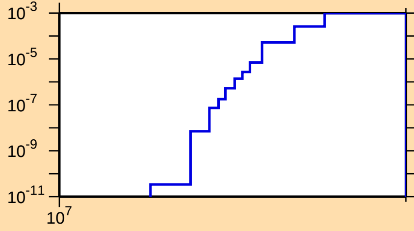
\sigma vs. E for ^{88}\text{Br}(n,np)
