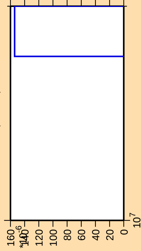
\Delta\sigma/\sigma vs. E for ^{88}\text{Br}(\text{mt 11})
