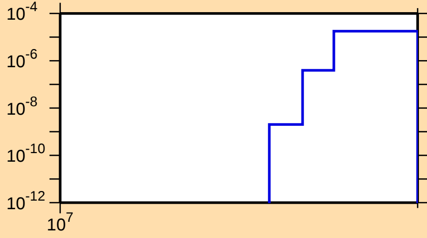
\sigma vs. E for ^{88}\text{Br}(n,nt)
