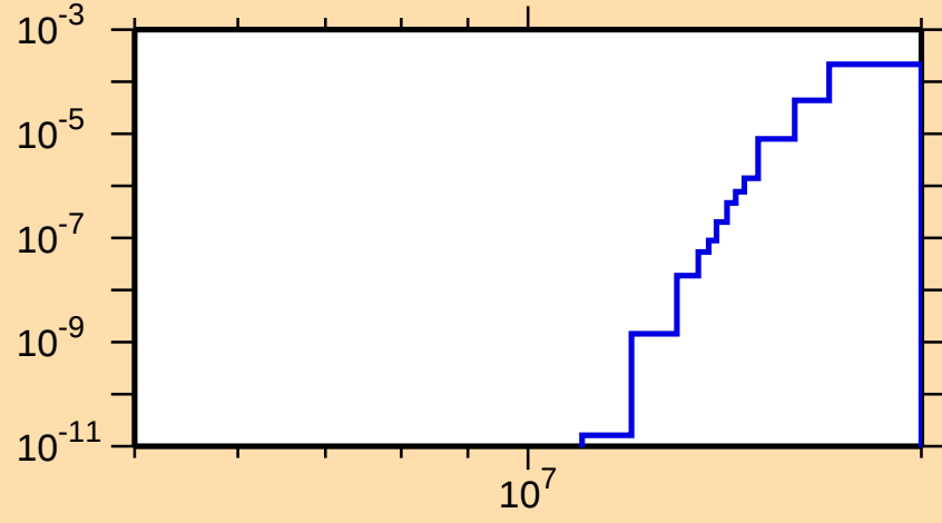
\sigma vs. E for ^{88}\text{Br}(n,n\alpha)
