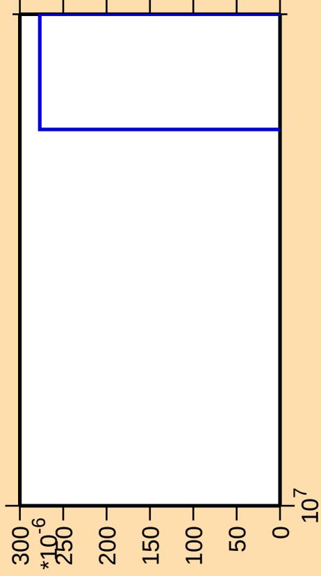
\Delta\sigma/\sigma vs. E for ^{88}\text{Br}(n,\text{He}3)
