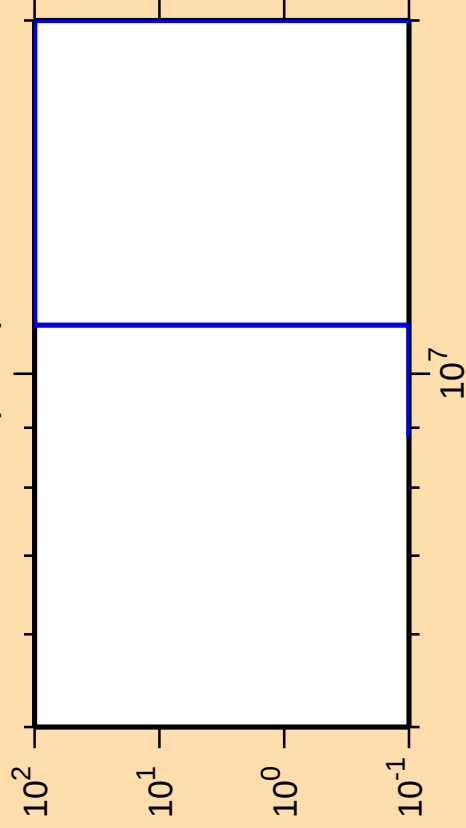
\Delta\sigma/\sigma vs. E for ^{88}\text{Br}(n,n\alpha)
