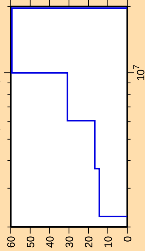
\Delta\sigma/\sigma vs. E for ^{88}\text{Br}(n,\text{ncont.})
