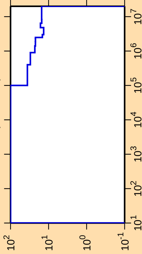
\Delta\sigma/\sigma vs. E for ^{88}\text{Br}(n,\text{nonel.})
