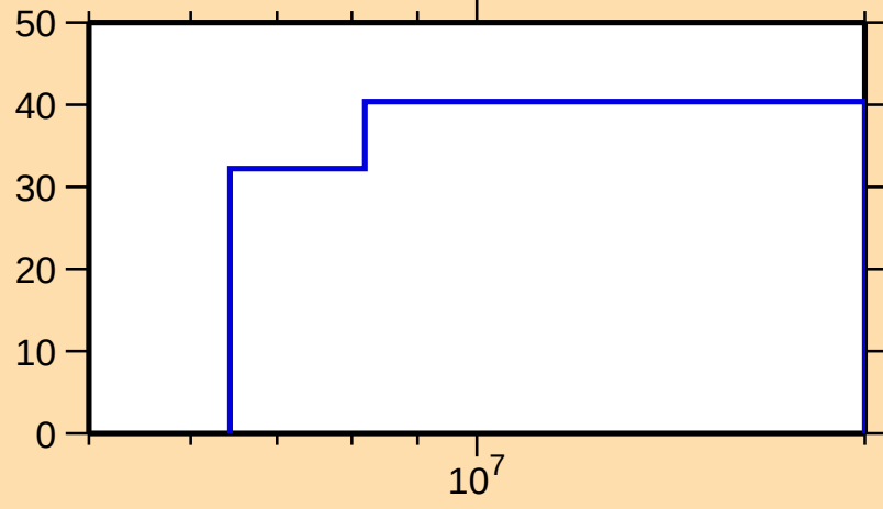
\Delta\sigma/\sigma vs. E for ^{88}\text{Br}(n,\text{inel.})
