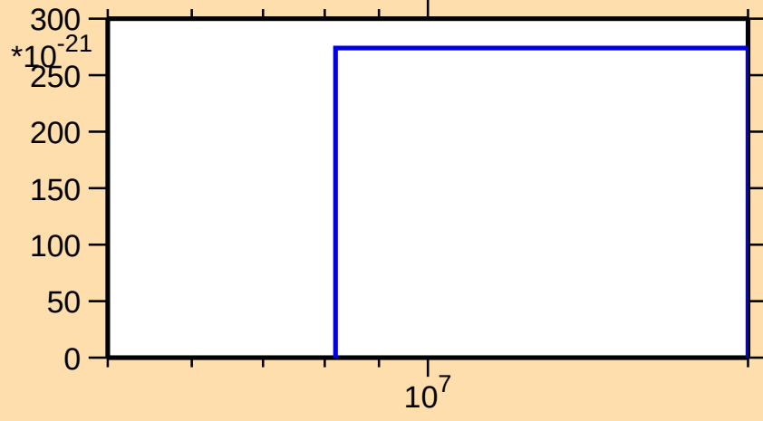
\sigma vs. E for ^{88}\text{Br}(n,\text{He}3)
