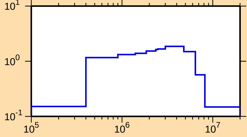
\sigma vs. E for ^{88}\text{Br}(n,\text{inel.})
