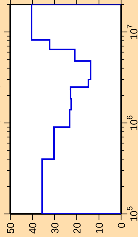
\Delta\sigma/\sigma vs. E for ^{88}\text{Br}(n,\text{inel.})
