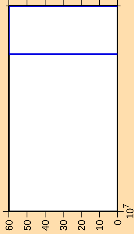
\Delta\sigma/\sigma vs. E for ^{89}\text{Br}(n,2np)
