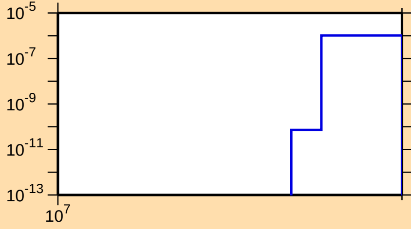
\sigma vs. E for ^{89}\text{Br}(n,\text{nd})
