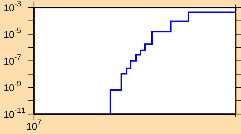
\sigma vs. E for ^{89}\text{Br}(n,np)
