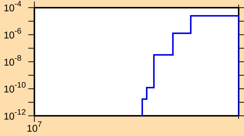
\sigma vs. E for ^{89}\text{Br}(n,nt)
