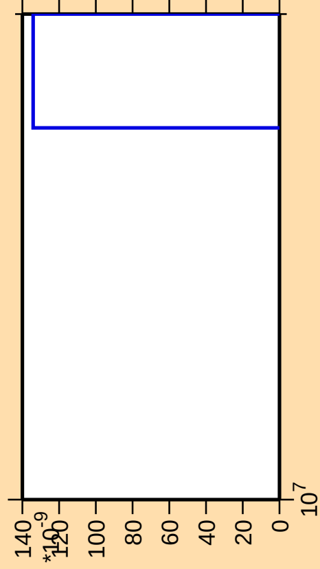
\Delta\sigma/\sigma vs. E for ^{89}\text{Br}(\text{mt 11})
