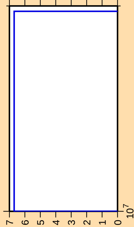
\Delta\sigma/\sigma vs. E for ^{89}\text{Br}(n,2np)
