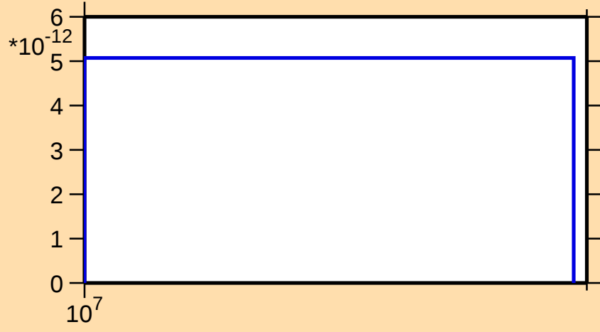
\sigma vs. E for ^{89}\text{Br}(n,2n\alpha)
