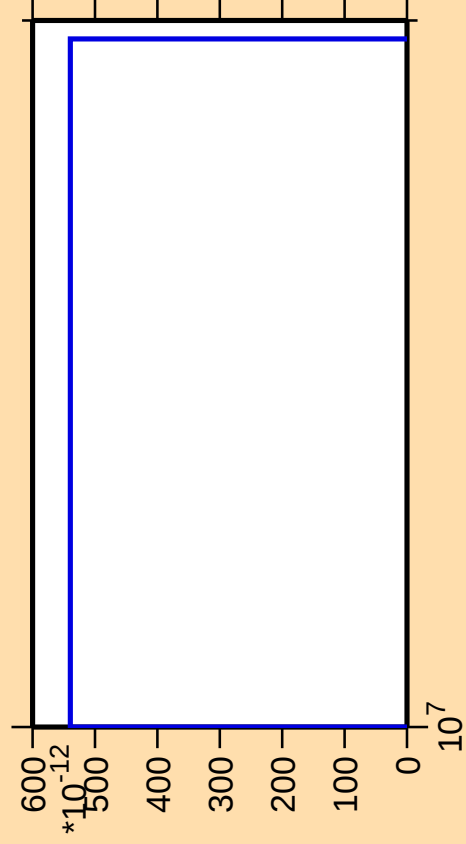
\Delta\sigma/\sigma vs. E for ^{89}\text{Br}(\text{mt 11})
