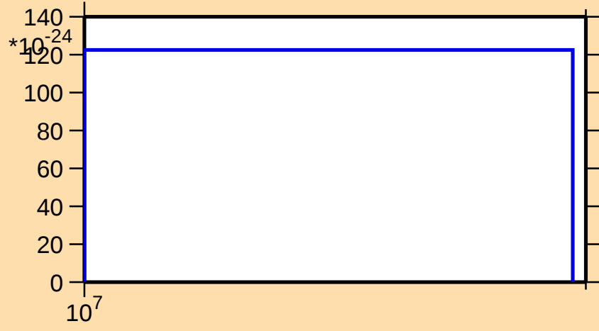
\sigma vs. E for ^{89}\text{Br}(\text{mt 11})
