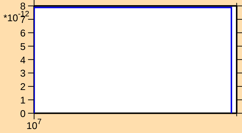
\sigma vs. E for ^{89}\text{Br}(n,2np)
