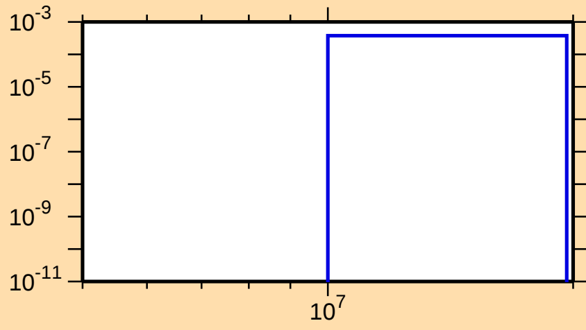
\sigma vs. E for ^{89}\text{Br}(n,p)
