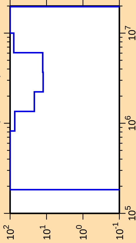
\Delta\sigma/\sigma vs. E for ^{89}\text{Br}(n,n_{\text{cont}})
