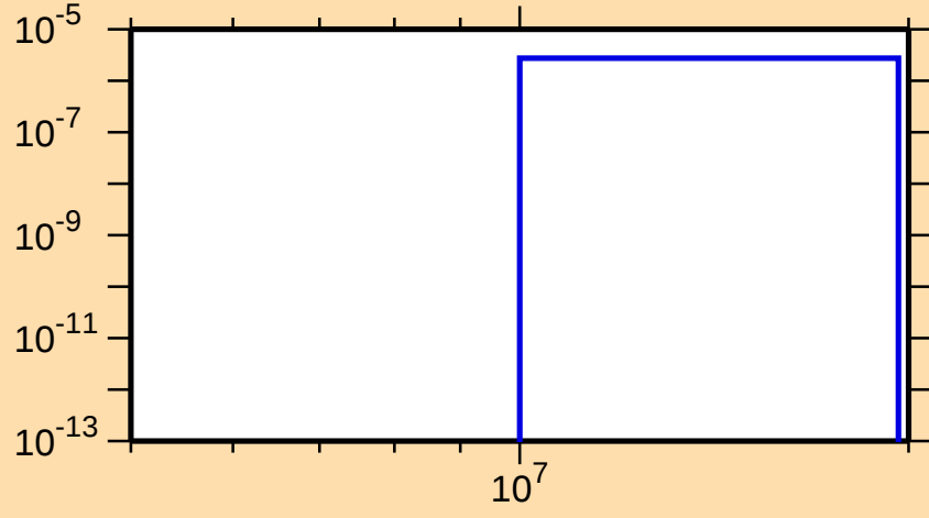
\sigma vs. E for ^{89}\text{Br}(n,n\alpha)
