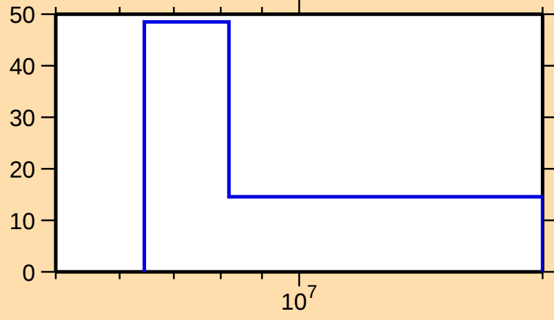
\Delta\sigma/\sigma vs. E for ^{89}\text{Br}(n,2n)
