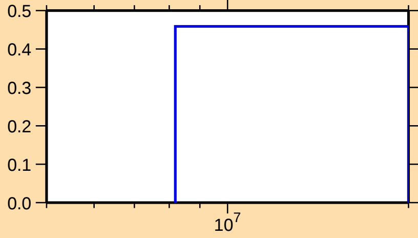
\sigma vs. E for ^{89}\text{Br}(n,3n)
