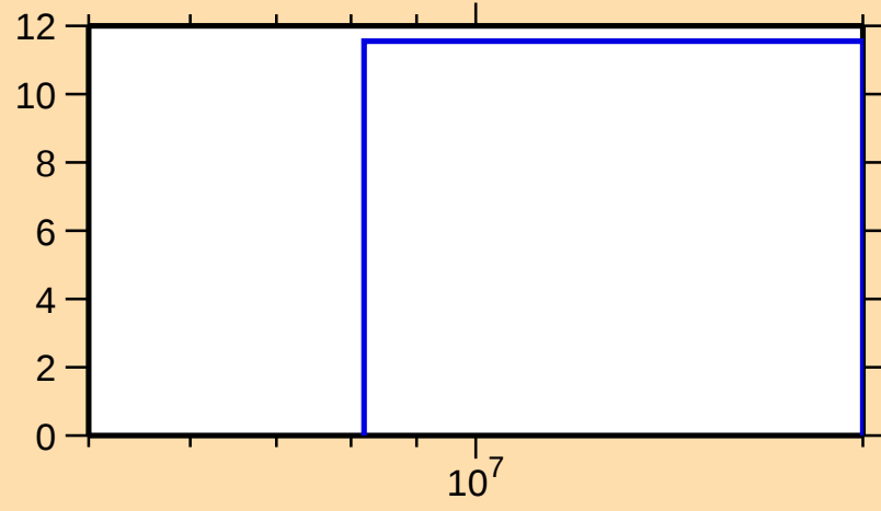
\Delta\sigma/\sigma vs. E for ^{89}\text{Br}(n,\text{nonel.})
