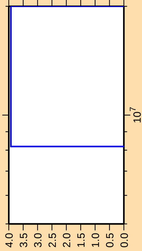
\Delta\sigma/\sigma vs. E for ^{89}\text{Br}(n,2n\alpha)
