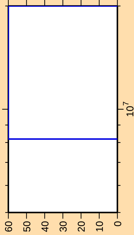
\Delta\sigma/\sigma vs. E for ^{89}\text{Br}(n,n\alpha)
