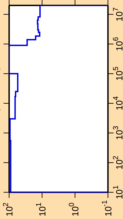
\Delta\sigma/\sigma vs. E for ^{89}\text{Br}(n,\text{nonel.})
