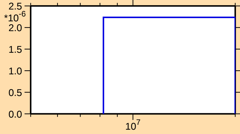
\sigma vs. E for ^{89}\text{Br}(n,n\alpha)
