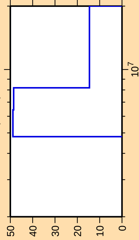
\Delta\sigma/\sigma vs. E for ^{89}\text{Br}(n,2n)
