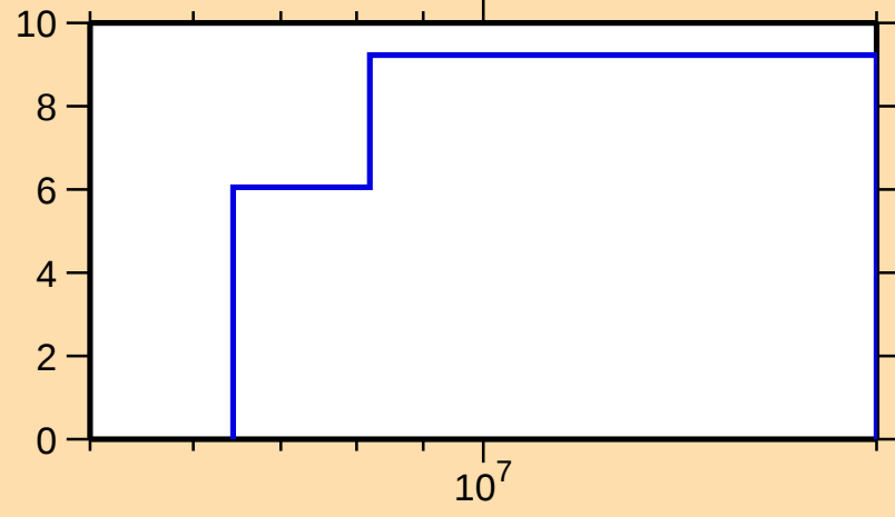
\Delta\sigma/\sigma vs. E for ^{89}\text{Br}(n,\text{tot.})
