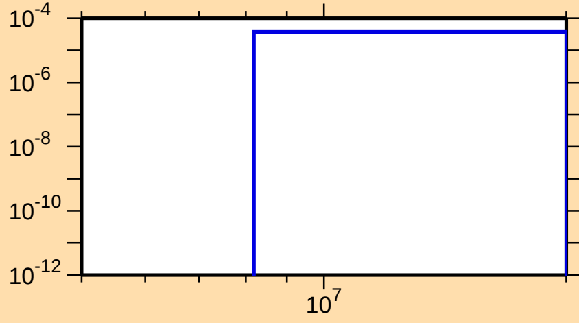
\sigma vs. E for ^{89}\text{Br}(n,\alpha)
