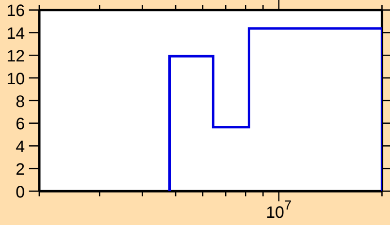
\Delta\sigma/\sigma vs. E for ^{89}\text{Br}(n,\text{el.})
