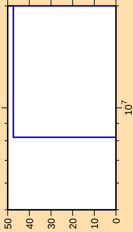
\Delta\sigma/\sigma vs. E for ^{89}\text{Br}(n,3n)
