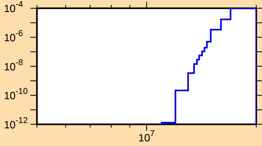
\sigma vs. E for ^{90}\text{Br}(n,n\alpha)
