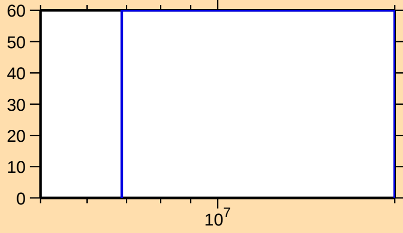
\Delta\sigma/\sigma vs. E for ^{90}\text{Br}(n,\text{inel.})
