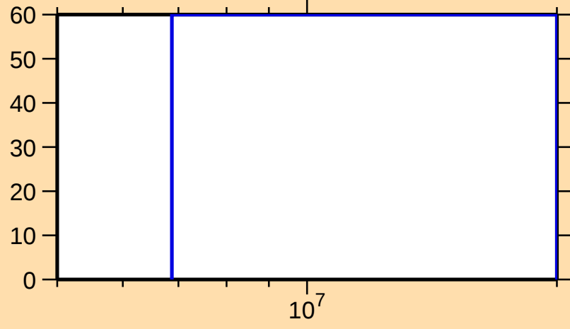
\Delta\sigma/\sigma vs. E for ^{90}\text{Br}(n,n\text{cont.})
