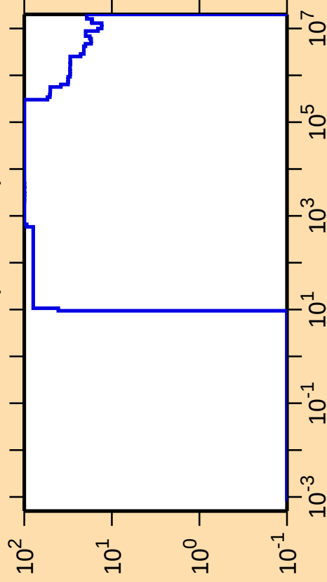
\Delta\sigma/\sigma vs. E for ^{90}\text{Br}(n,\text{nonel.})
