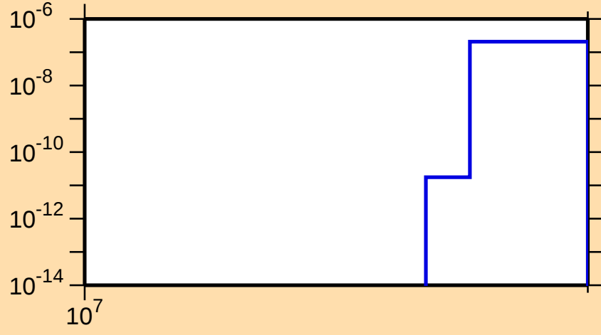
\sigma vs. E for ^{90}\text{Br}(n,2np)
