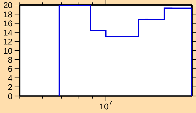
\Delta\sigma/\sigma vs. E for ^{90}\text{Br}(n,\text{nonel.})
