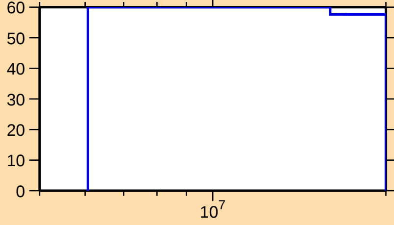
\Delta\sigma/\sigma vs. E for ^{90}\text{Br}(n,\gamma)
