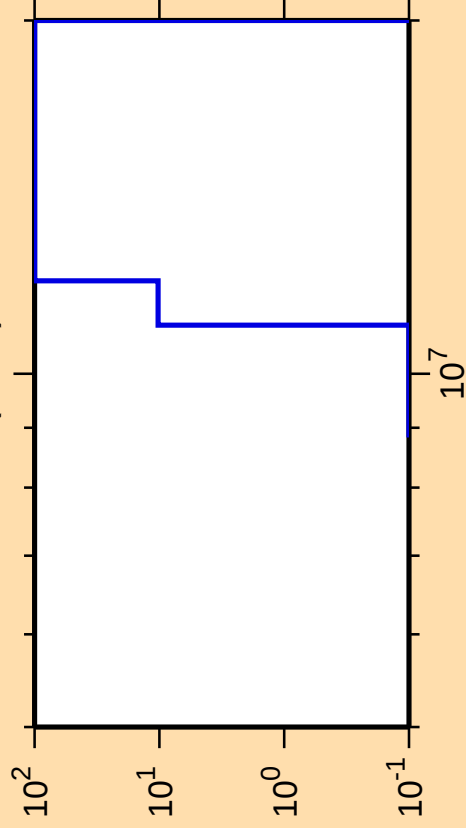
\Delta\sigma/\sigma vs. E for ^{90}\text{Br}(n,n\alpha)
