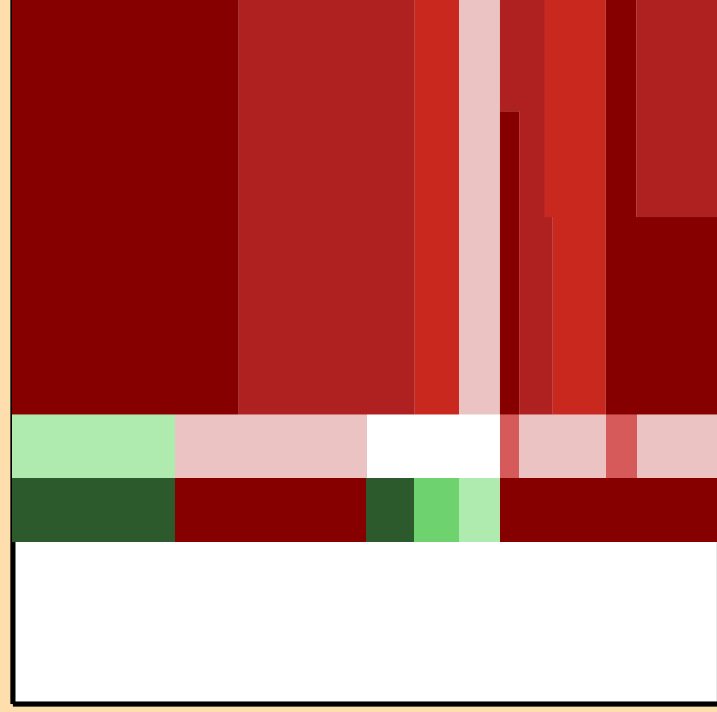
\Delta\sigma/\sigma vs. E for ^{90}\text{Br}(n,n_1)
