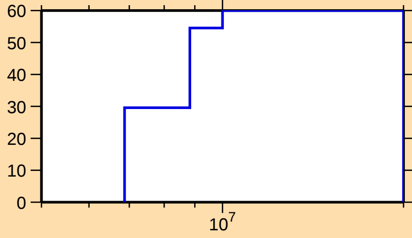
\Delta\sigma/\sigma vs. E for ^{90}\text{Br}(n,2n)
