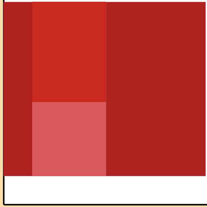
\Delta\sigma/\sigma vs. E for ^{90}\text{Br}(n,n\text{cont.})
