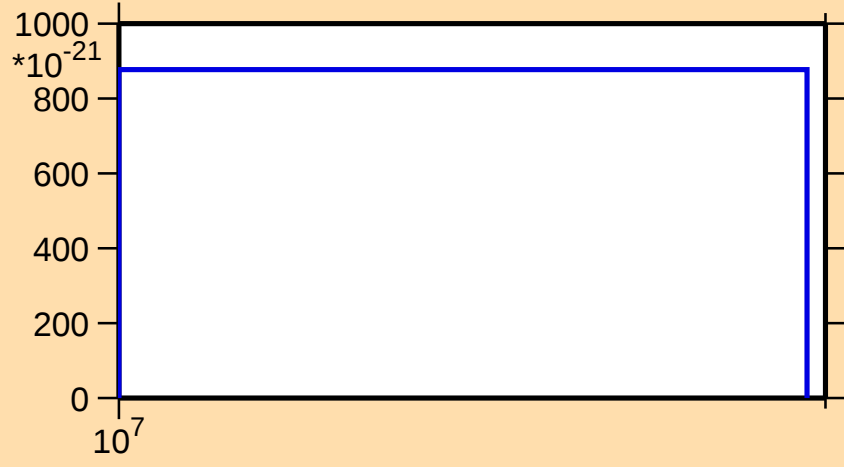
\sigma vs. E for ^{90}\text{Br}(\text{mt 11})
