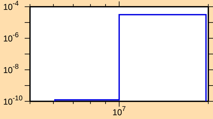
\sigma vs. E for ^{90}\text{Br}(n,\alpha)
