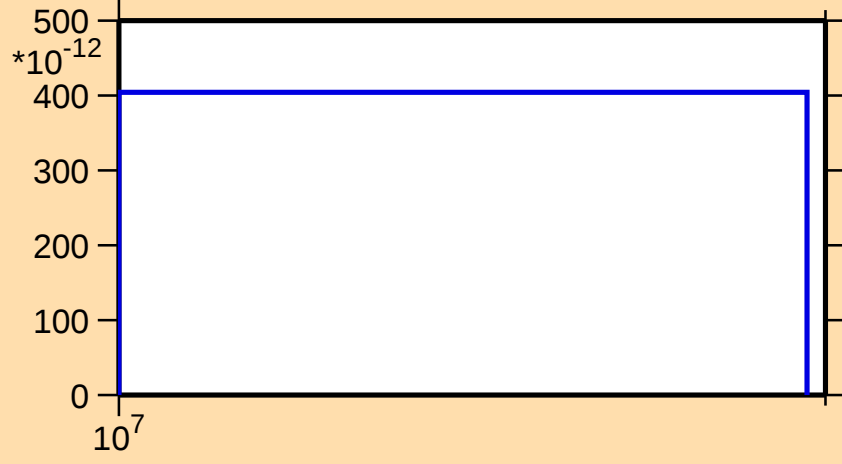
\sigma vs. E for ^{90}\text{Br}(n,2n\alpha)
