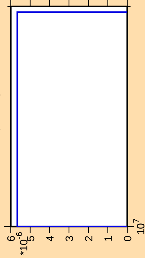
\Delta\sigma/\sigma vs. E for ^{90}\text{Br}(\text{mt 11})
