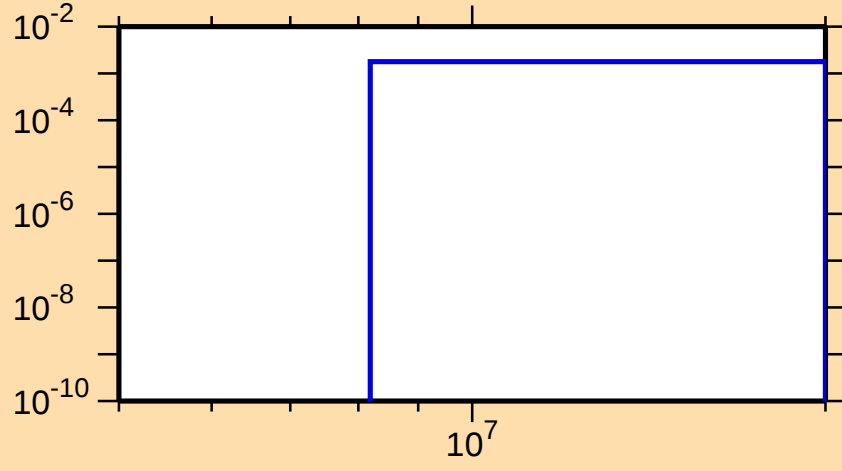
\sigma vs. E for ^{90}\text{Br}(n,p)
