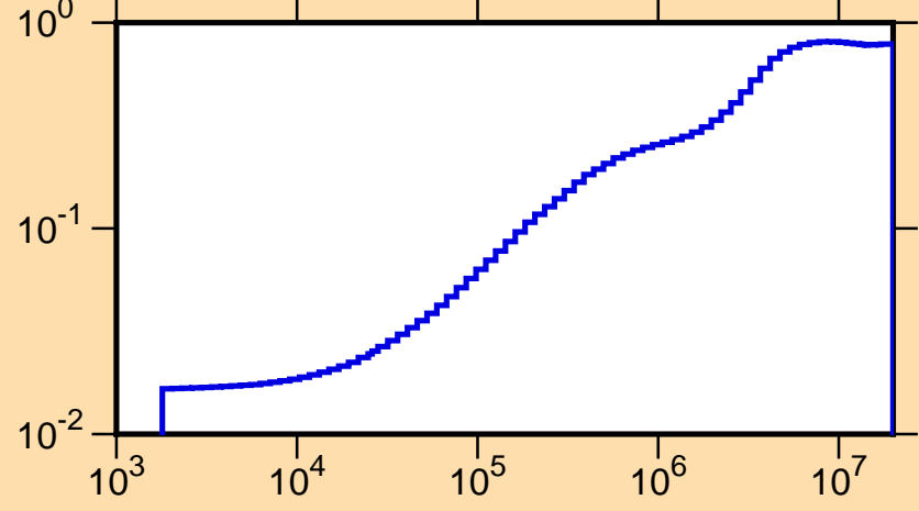
\mu vs. E for ^{41}\text{Ca}(\text{mt251})
