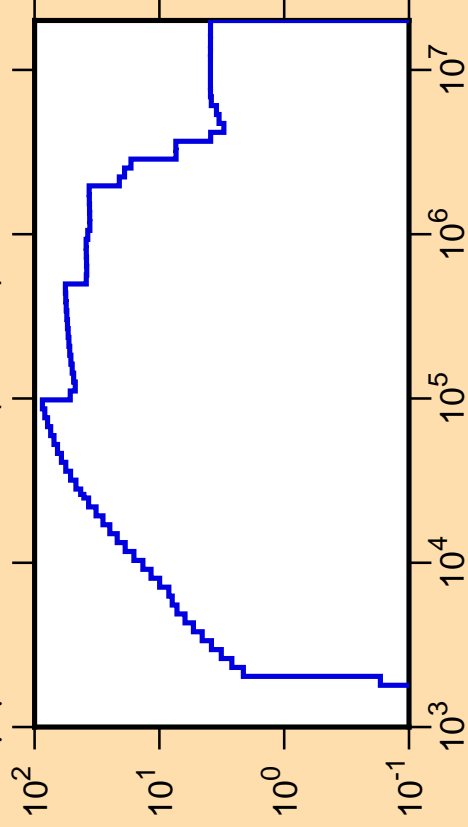
\Delta\mu/\mu vs. E for ^{41}\text{Ca}(\text{mt251})
